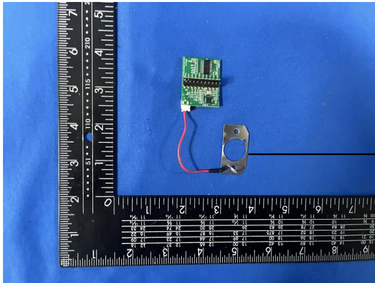
315MHz Internal Antenna
