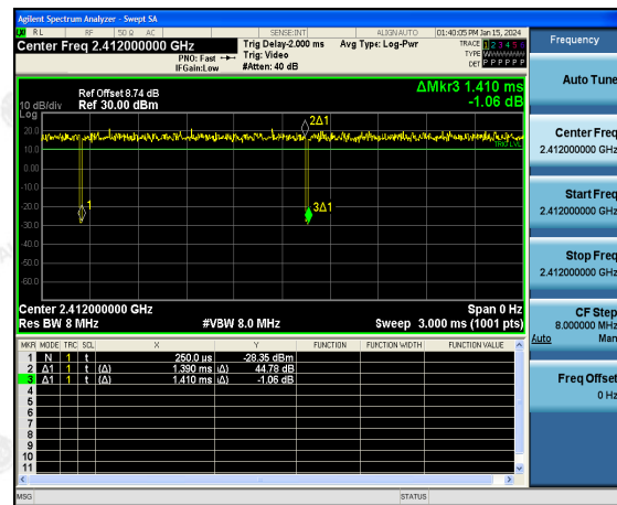
802.11g
