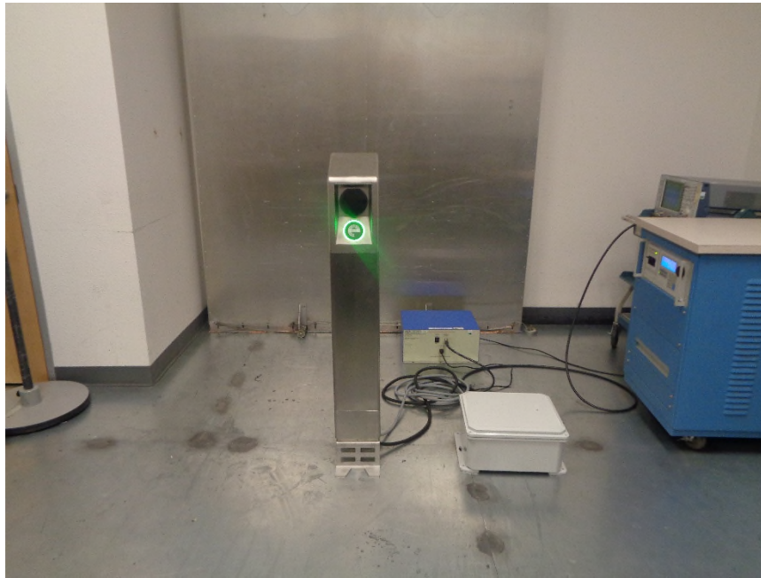
Figure 9: Conducted Emissions Front View
