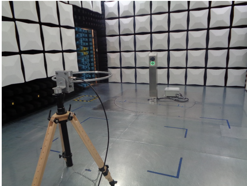
Figure 5: Polarization Z-Axis Front View
