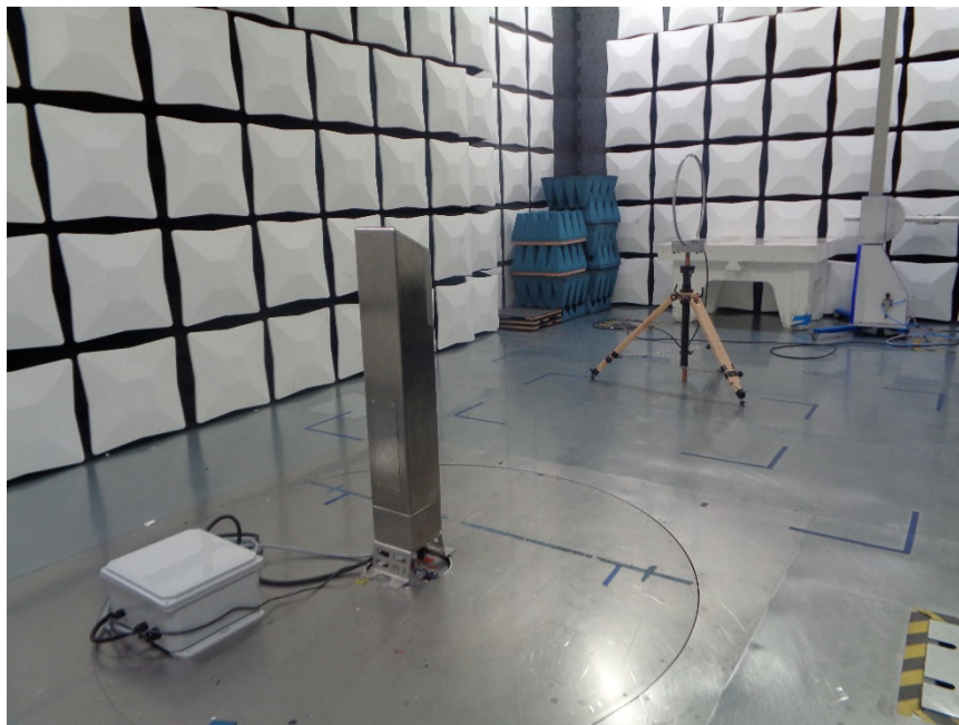
Figure 4: Polarization Y-Axis Back View
