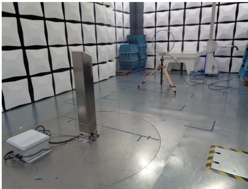
Figure 2: Polarization X-Axis Back View
