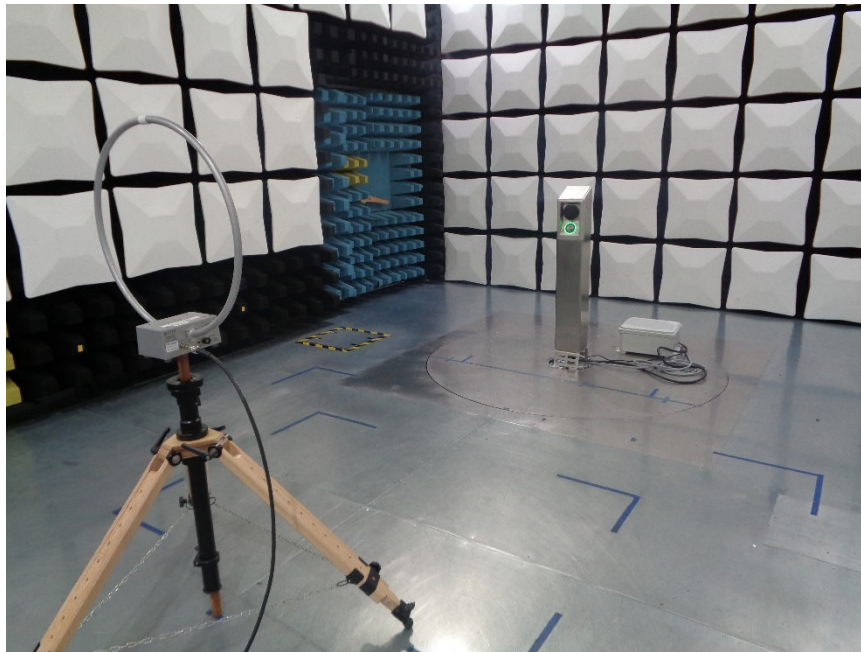
Figure 1: Polarization X-Axis Front View
