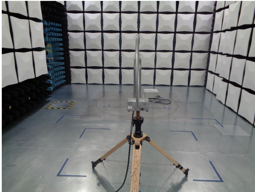
Figure 3: Polarization Y-Axis Front View
