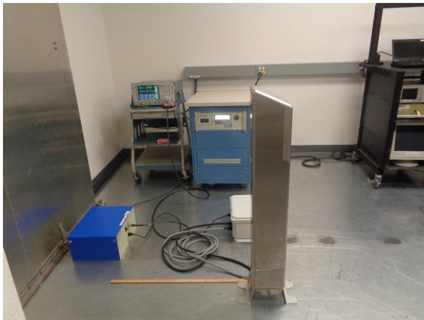
Figure 10: Conducted Emissions Side View
