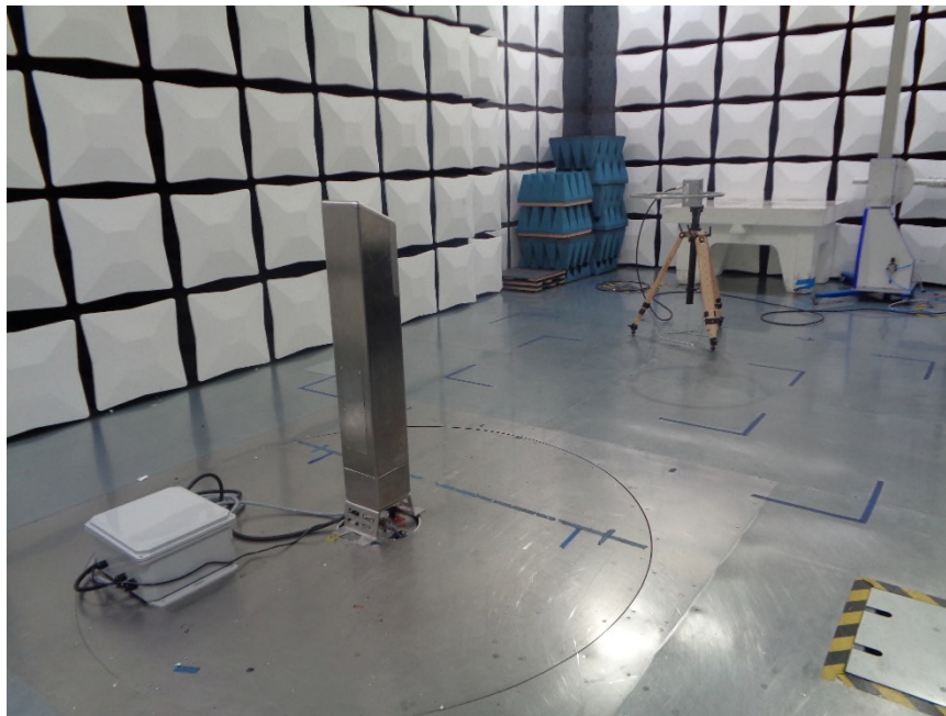
Figure 6: Polarization Z-Axis Back View
