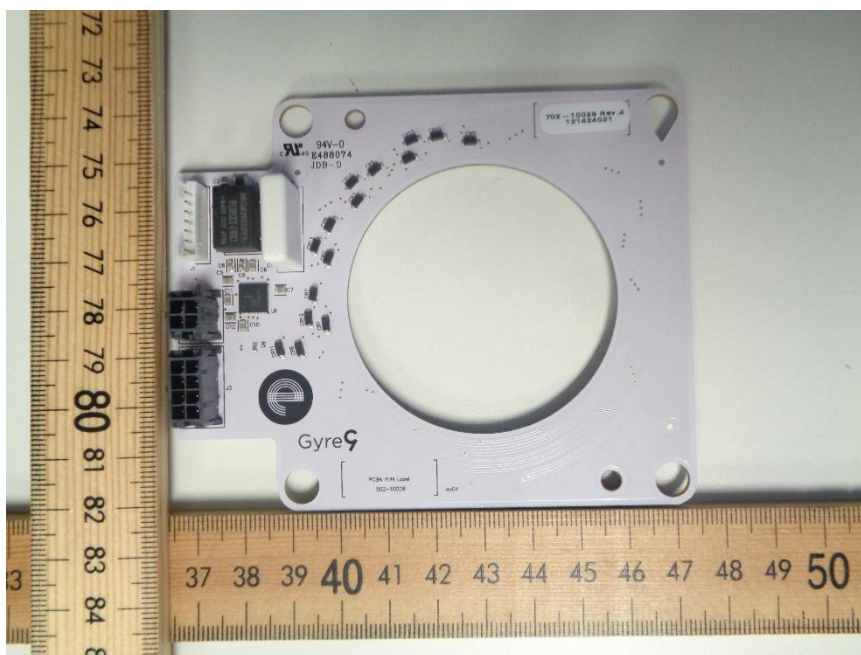
Figure 8 - PCB 1 Top
