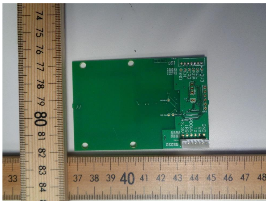
Figure 12 - PCB 2 Bottom
