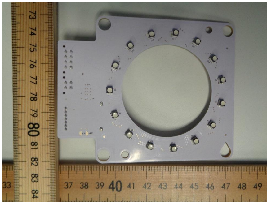
Figure 9 - PCB 1 Bottom
