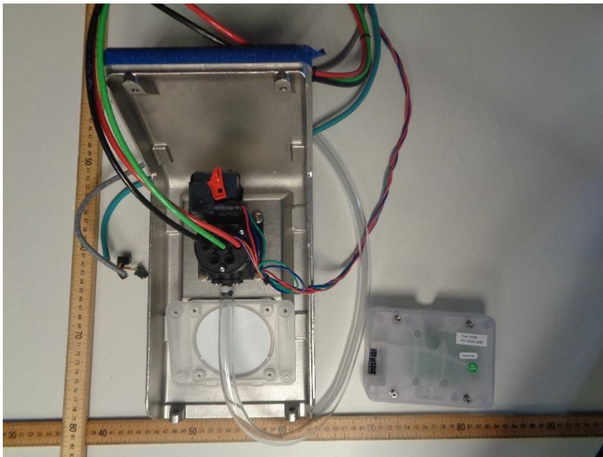
Figure 3 - Top of EUT
