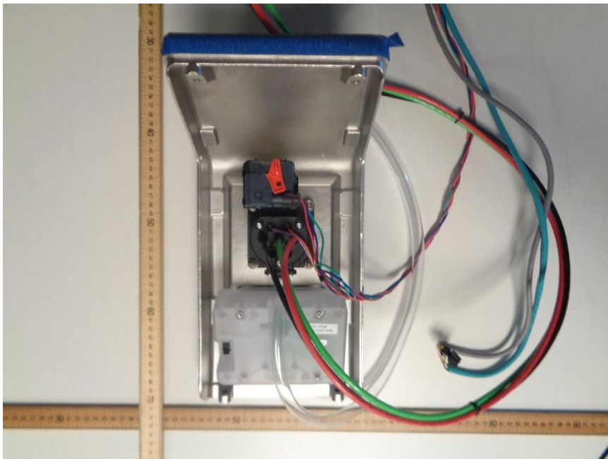
Figure 2 - Top of EUT
