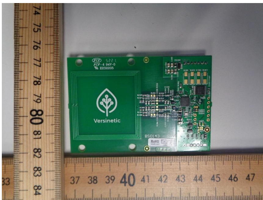
Figure 10 - PCB 2 Top
