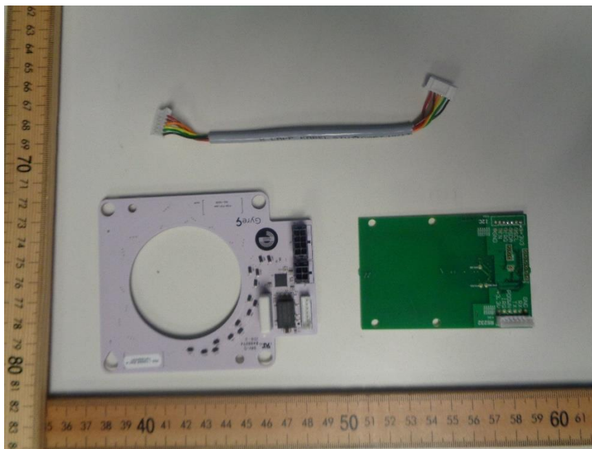
Figure 7 - PCB 1 & 2
