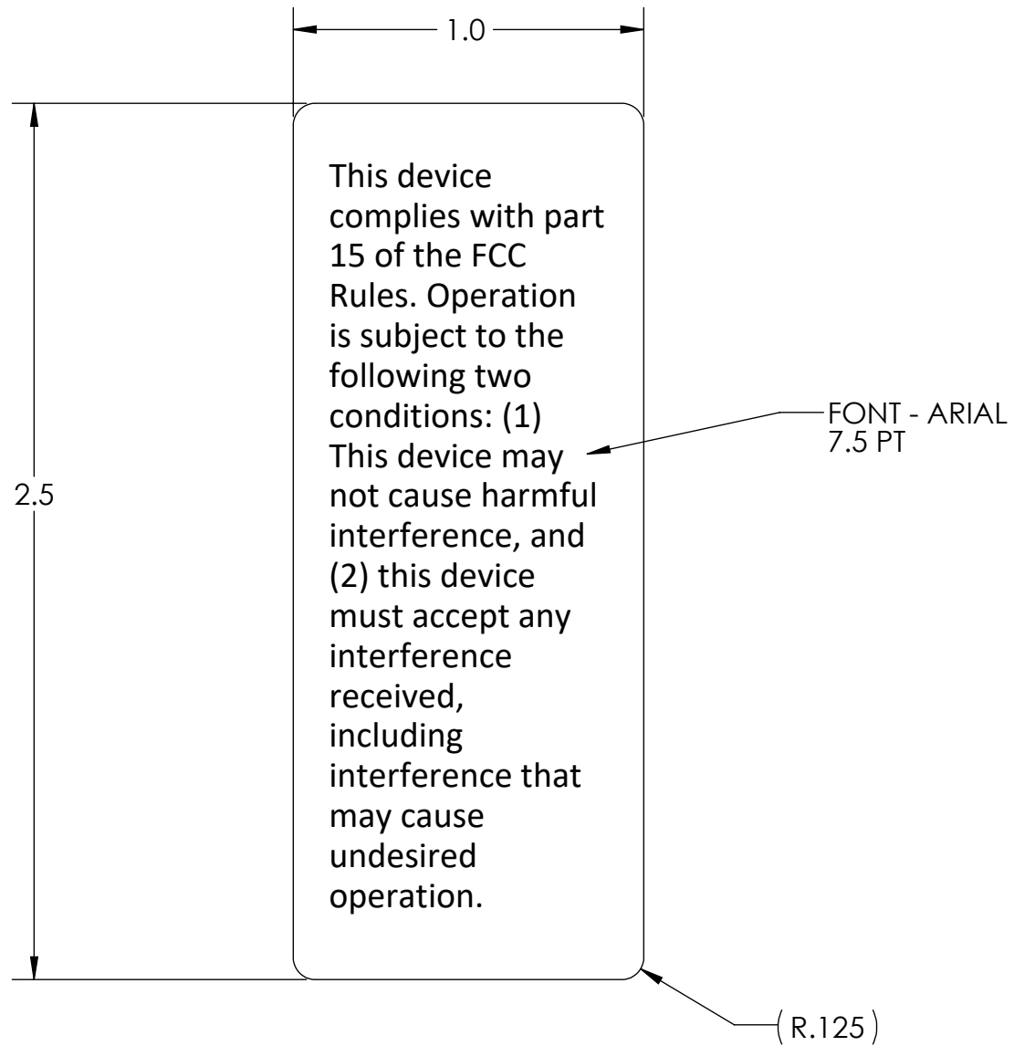
LABEL DETAILS
