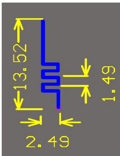
AntennaPhoto&Length (mm)
