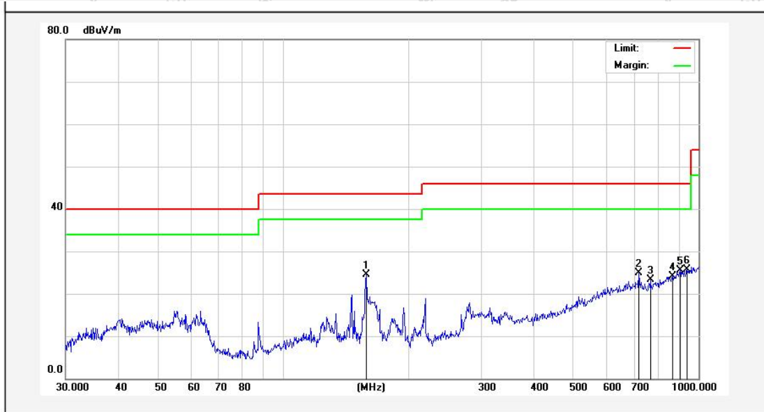
TM1 / Polarization: Horizontal / Band: 2400-2483.5 MHz
