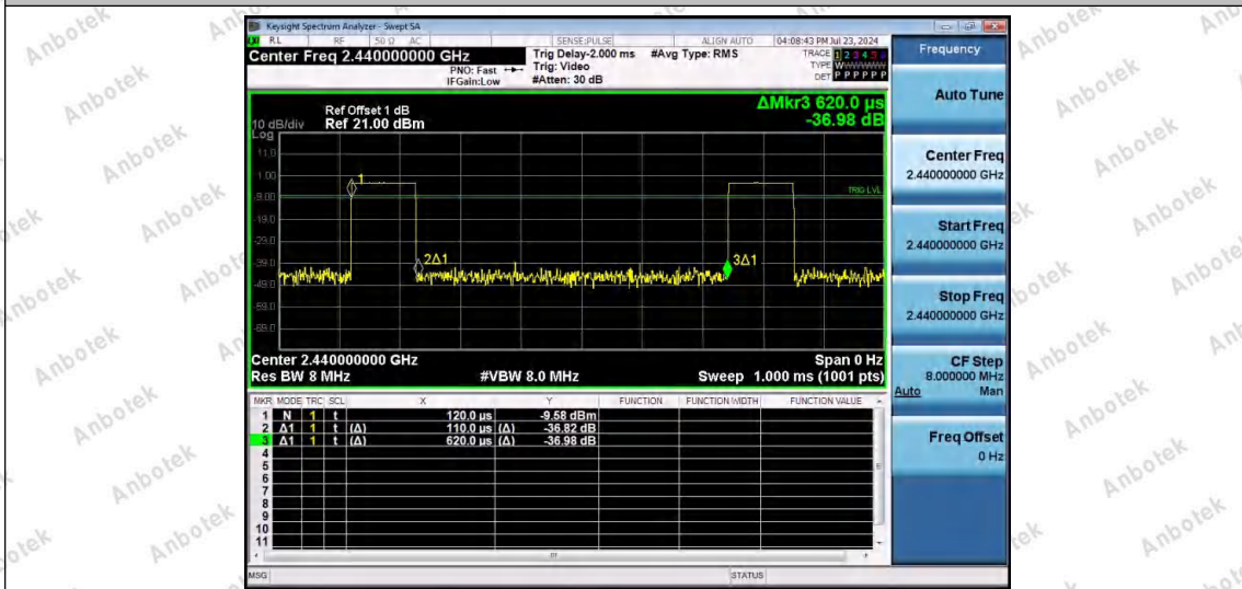
NTNV-BLE_1M-Ant1-2440
