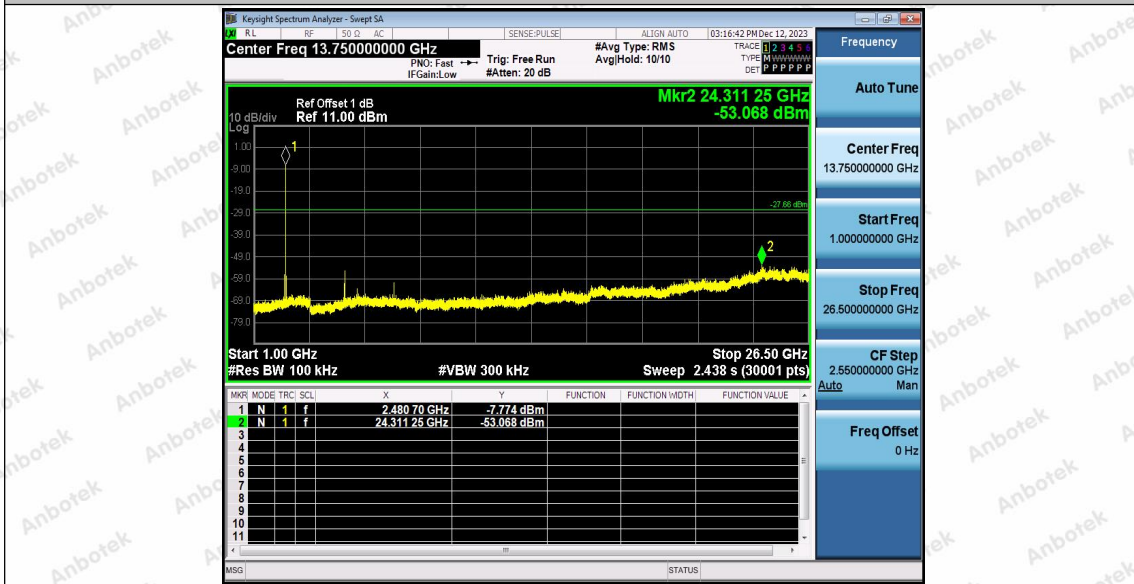
2.4G_Ant1_2480.65_1000~26500
