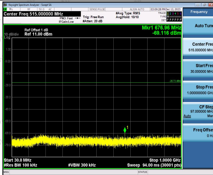
2.4G_Ant1_2441.65_30~1000
