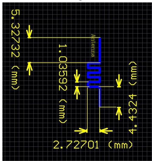
AntennaPhoto&Length (mm)
