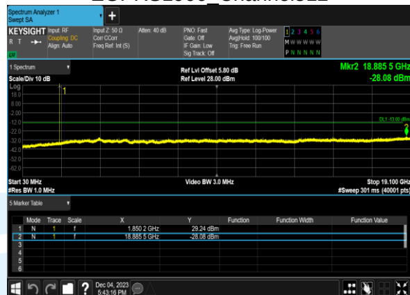
EGPRS1900 Channel512
