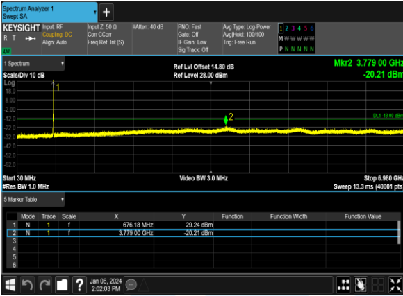
B71_10M_QPSK_1@0_CH_133422
