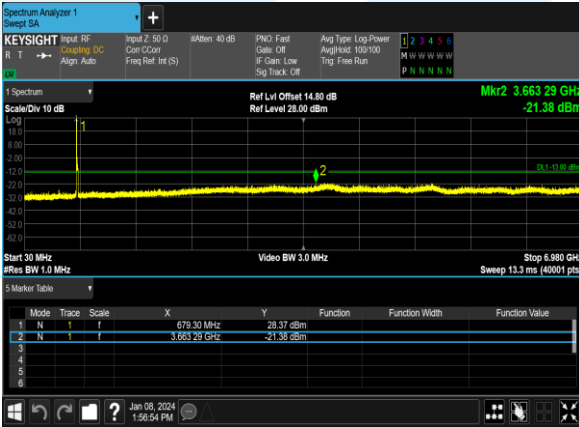
B71_20M_QPSK_1@0_CH_133372
