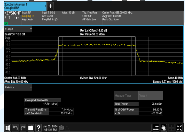
B71_20M_16QAM_100@0_CH_133372
