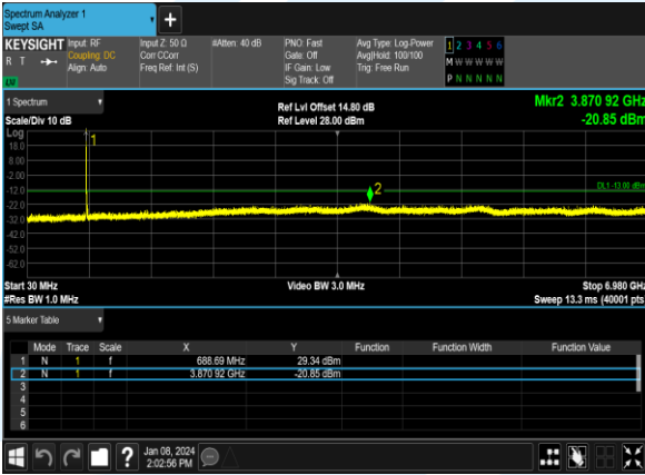
B71_5M_QPSK_1@0_CH_133147
