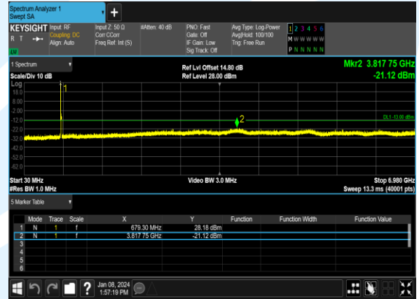
B71_20M_16QAM_1@0_CH_133372
