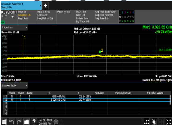
B71_5M_QPSK_1@0_CH_133297
