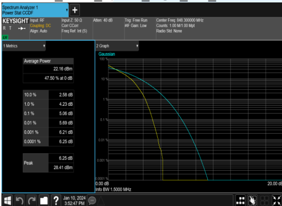
B26_1.4M_QPSK_6@0_CH_27033
