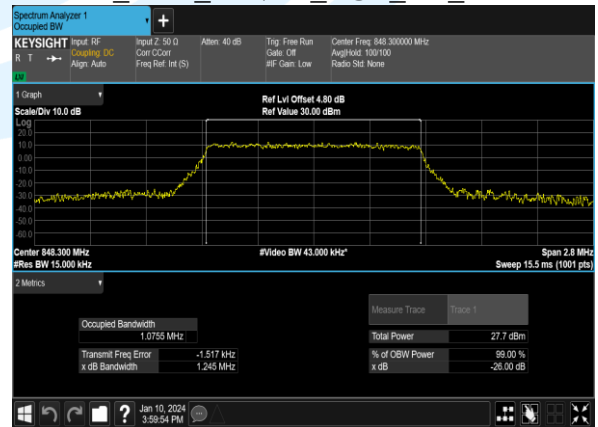
B26_1.4M_16QAM_6@0_CH_27033
