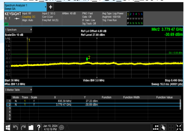
B26_3M_16QAM_1@0_CH_26915
