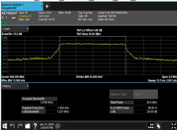
B26_1.4M_QPSK_6@0_CH_27033
