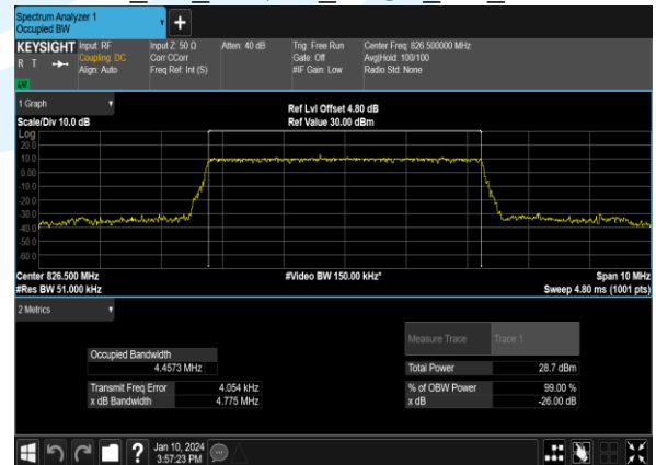
B26_5M_16QAM_25@0_CH_26815
