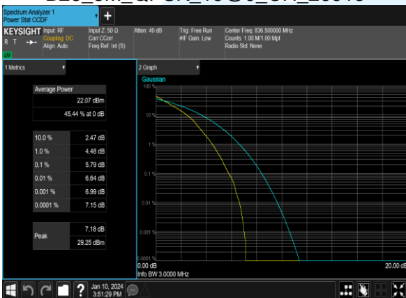
B26_3M_QPSK_15@0_CH_26915
