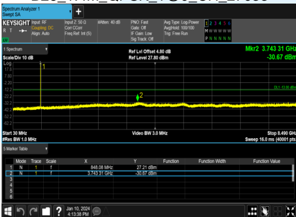
B26_1.4M_QPSK_1@0_CH_27033
