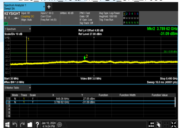
B26_1.4M_16QAM_1@0_CH_27033
