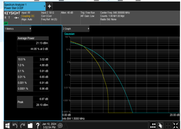
B26_1.4M_16QAM_6@0_CH_27033
