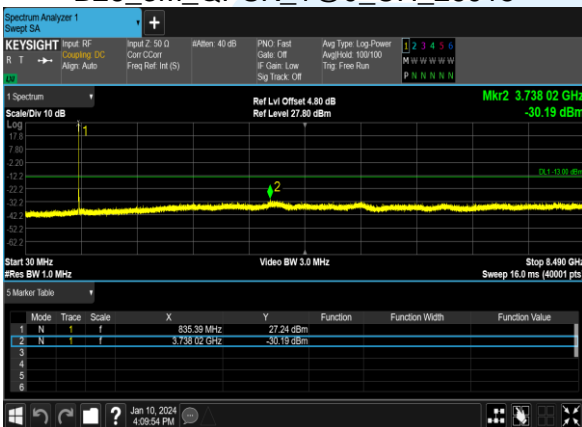
B26_3M_QPSK_1@0_CH_26915
