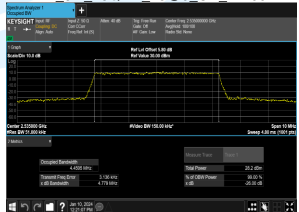
B7_5M_16QAM_25@0_CH_21100
