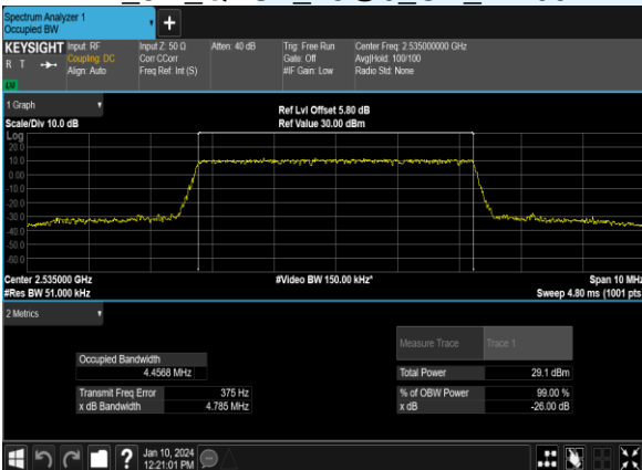
B7_5M_QPSK_25@0_CH_21100
