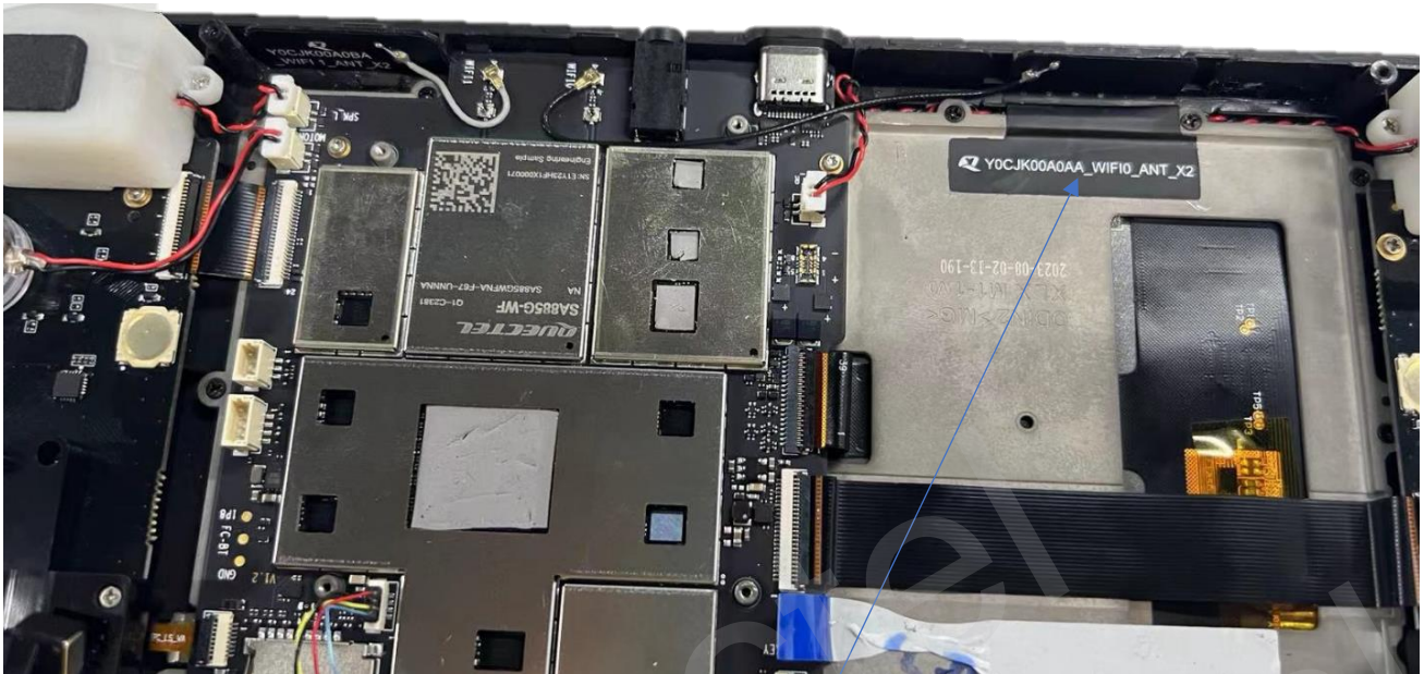
Antenna installation
