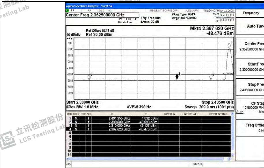
2DH5_Ant_Low_2402_Peak
