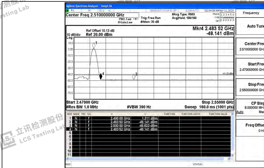
3DH5_Ant_High_2480_Peak
