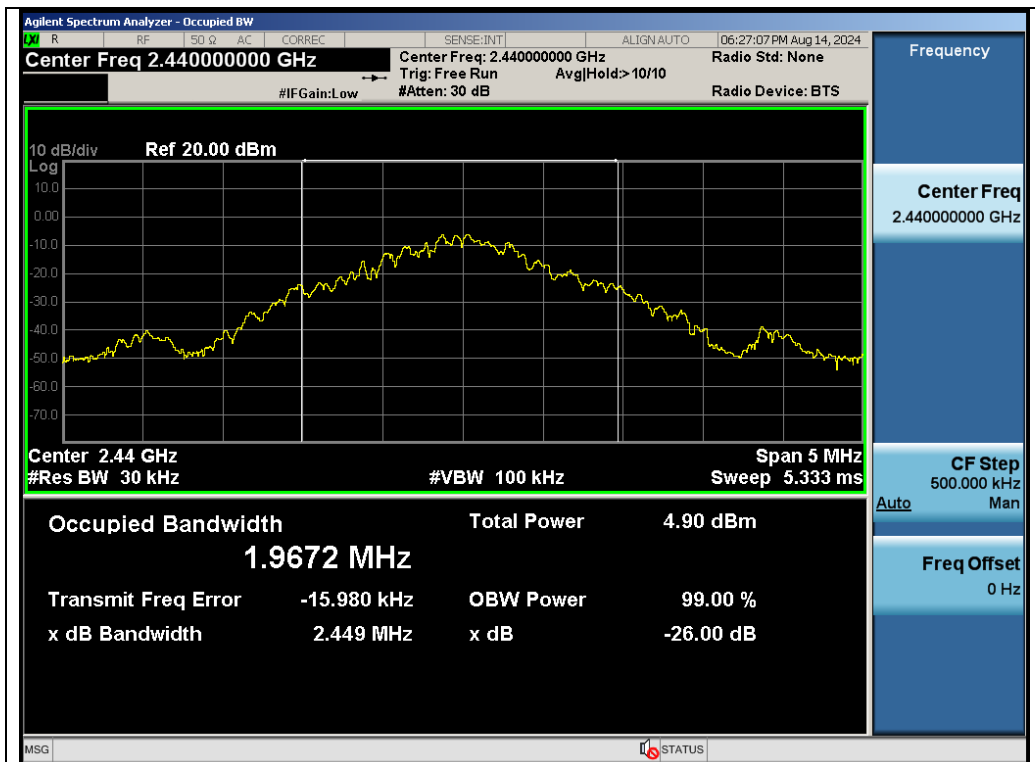
Test_Graph_2.4G_ANT1_2440_OBW
