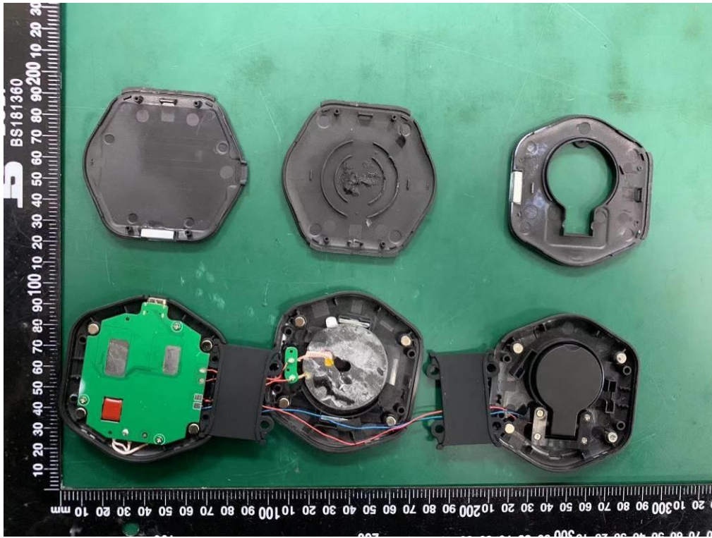
Internal Photo FCC ID: 2BDW6XB-WL301
