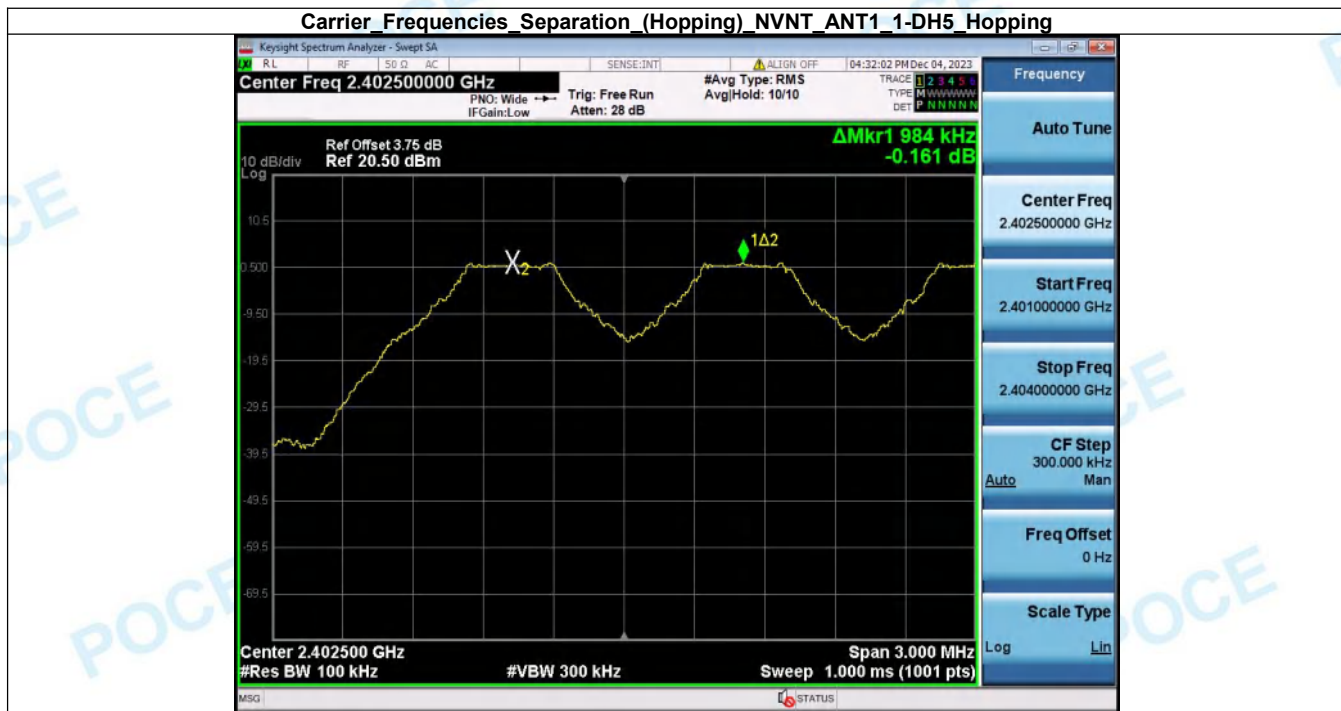
Carrier_Frequencies_Separation_(Hopping)_NVNT_ANT1_1-DH5_Hopping
