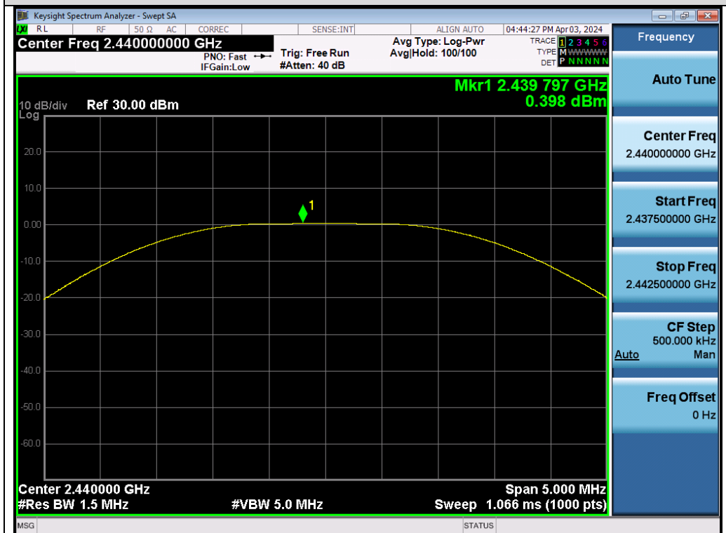
Test_Graph_GFSK_ANT1_2440_Peak Power
