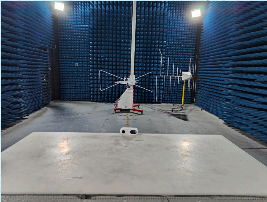
Radiated Emission Below 1GHz Test Setup
