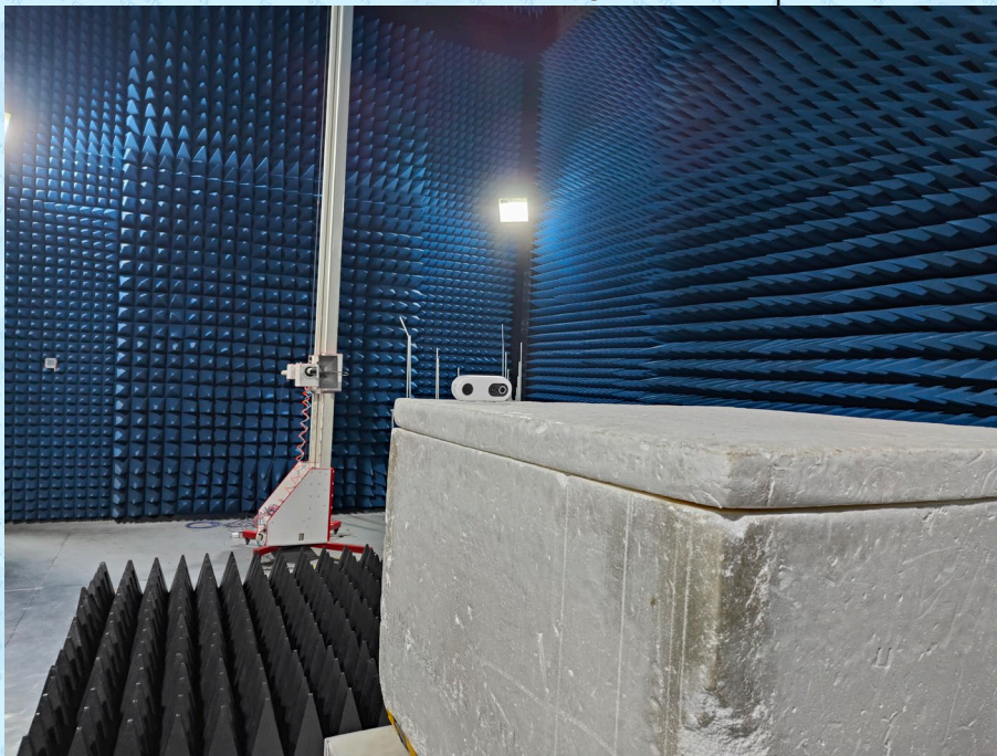
Radiated Emission Above 1GHz Test Setup
