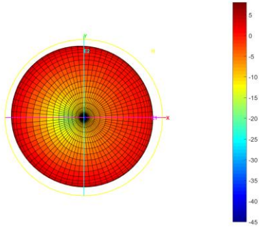
Total_3D_H_2.45GHz
