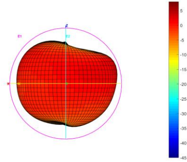
Total_3D_E1_2.45GHz
