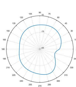
Total_Polar_E1_2.45GHz
