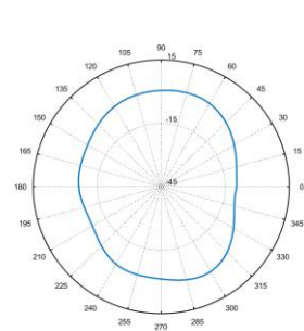
Total_Polar_E2_2.45GHz
