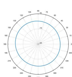
Total_Polar_H_2.45GHz
