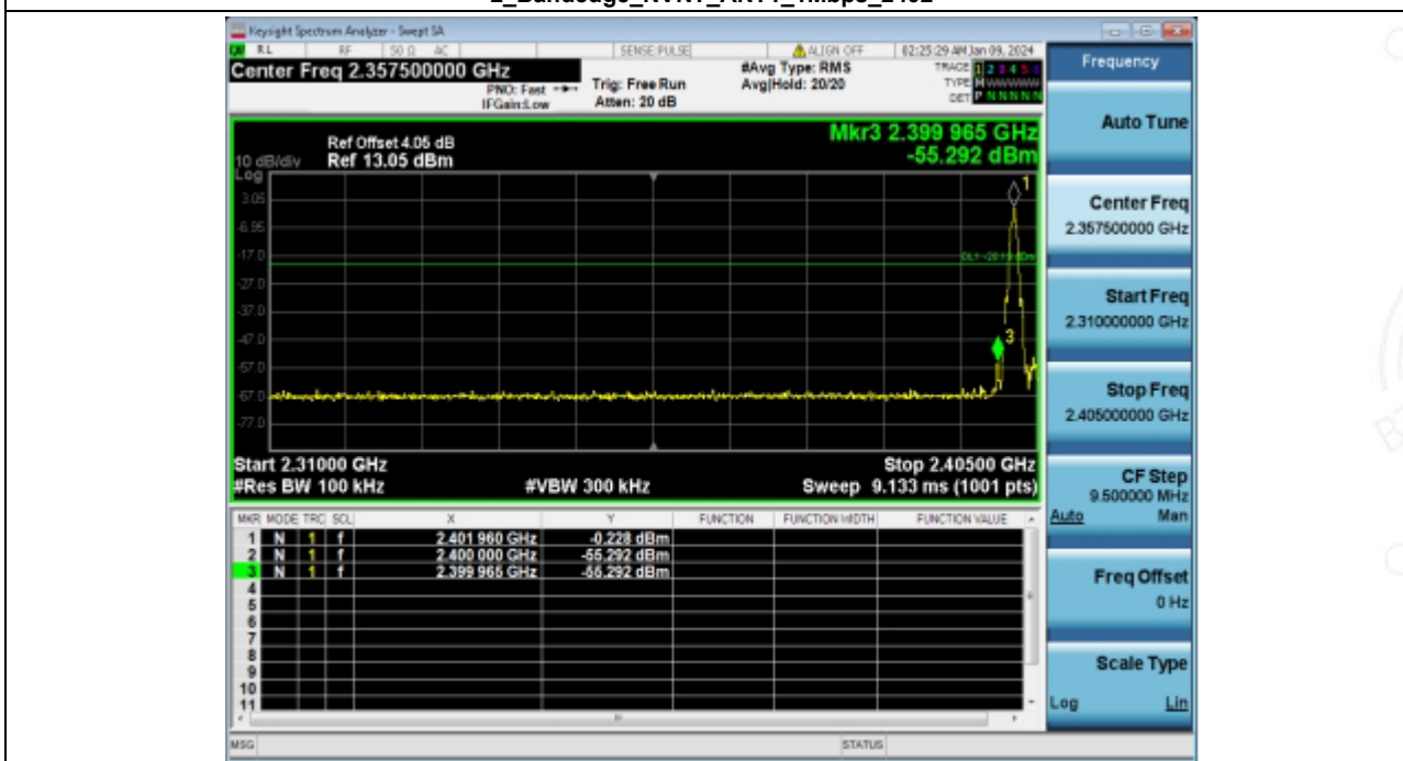
2_Bandedge_NVNT_ANT1_1Mbps_2402
