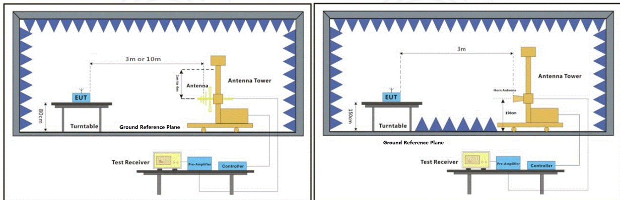
30MHz-1GHz
