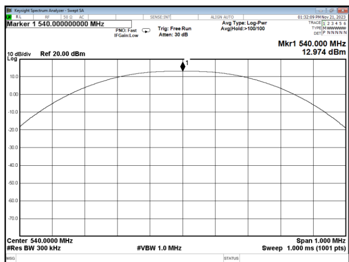
Channel 1 / 540.00 MHz
