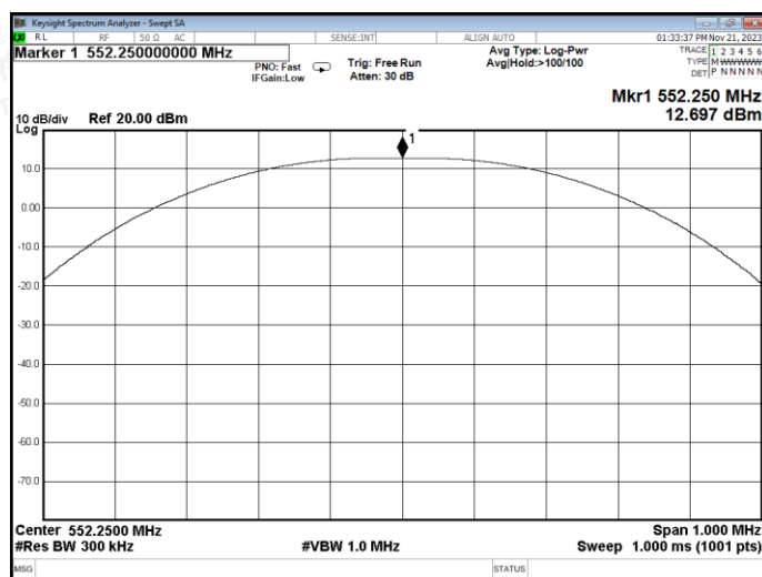
Channel 20 / 552.25 MHz
