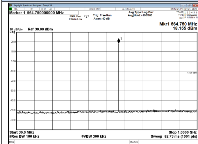
Channel 100 / 564.75 MHz
