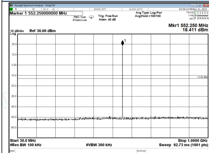
Channel 50 / 552.25 MHz
