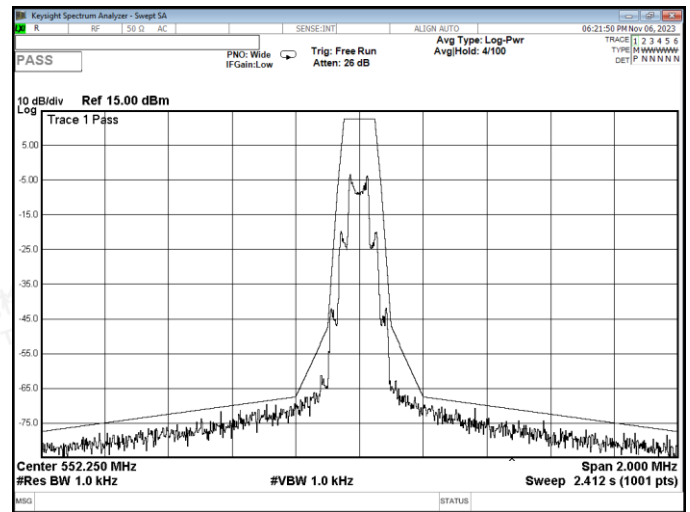
Channel 50 / 552.25 MHz
