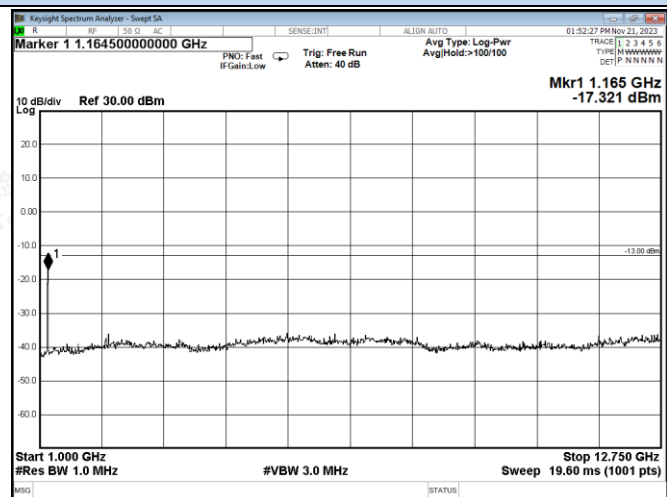
Channel 100 / 564.75 MHz
