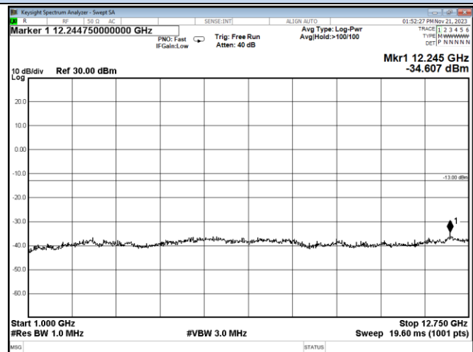
Channel 50 / 552.25 MHz
