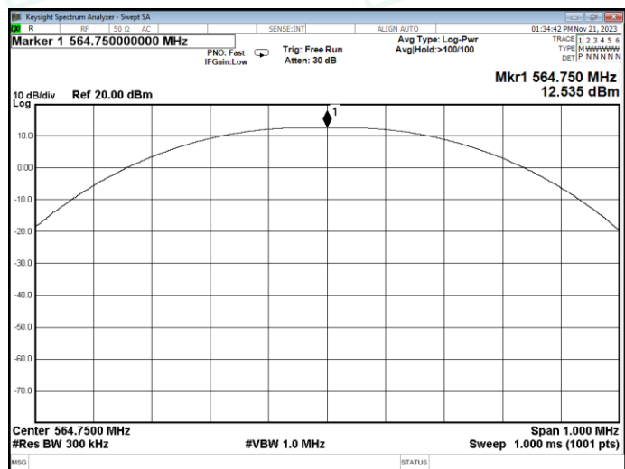
Channel 100 / 564.75 MHz
