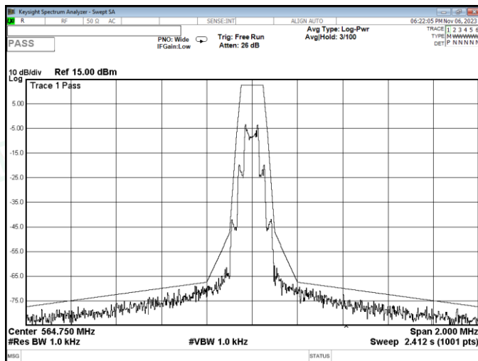
Channel 100 / 564.75 MHz
