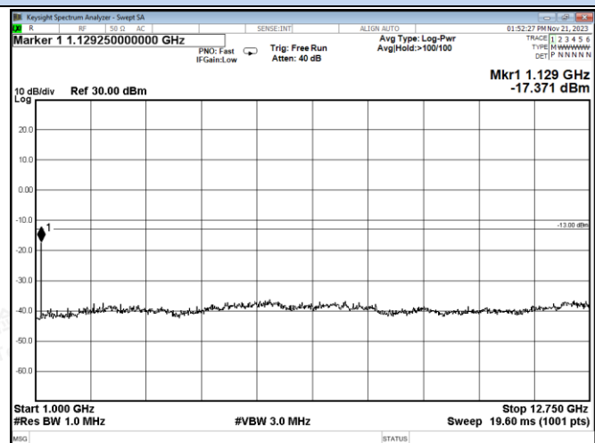
Channel 1 / 540.00 MHz
