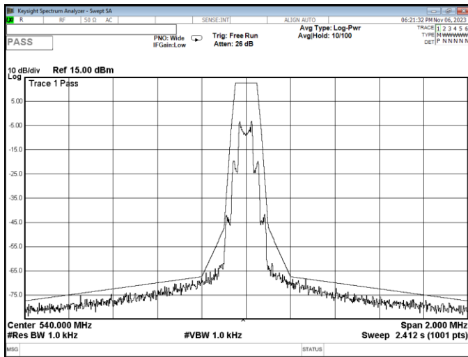
Channel 1 / 540.00 MHz
