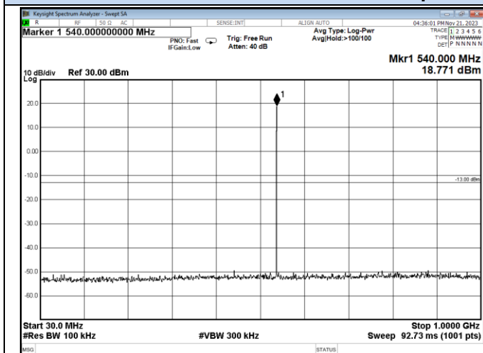
Channel 1 / 540.00 MHz
