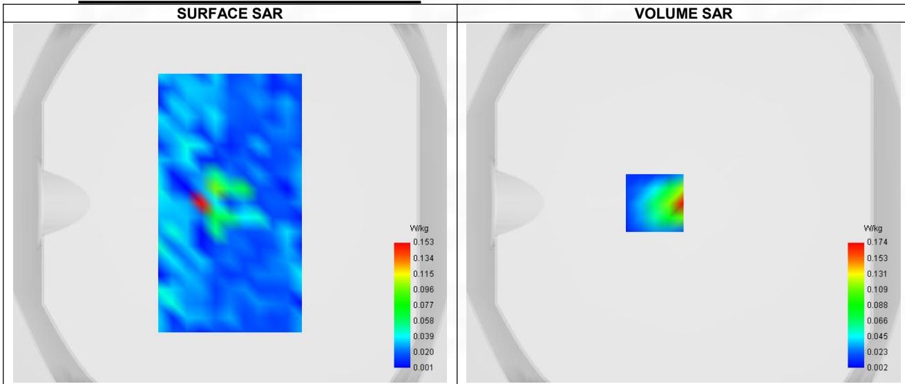
Maximum location: X=-16.00, Y=0.00 ; SAR Peak: 0.44 W/kg
