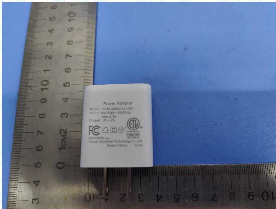
Photo 8 Adapter Appearance 2#
