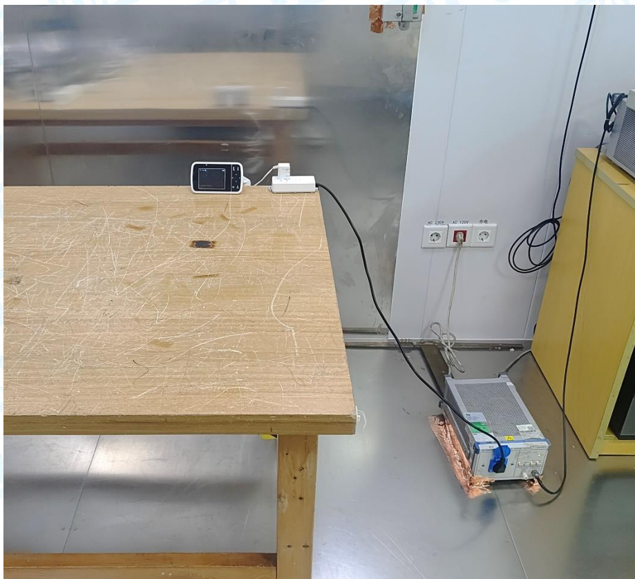
Photo of Setup for Conducted Emission
