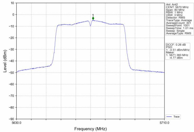
802.11ac(VHT40)_HCH_5670MHz_MIMO_NTNV
