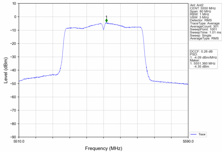
802.11ac(VHT40)_MCH_5550MHz_MIMO_NTNV
