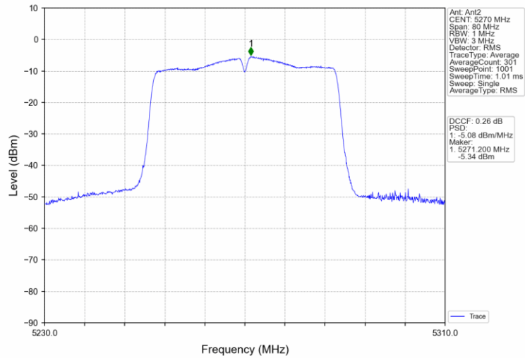
802.11ac(VHT40)_LCH_5270MHz_MIMO_NTNV
