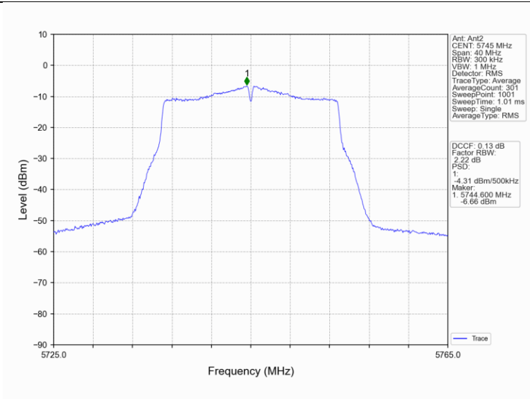
802.11n(HT20)_LCH_5745MHz_MIMO_NTNV
