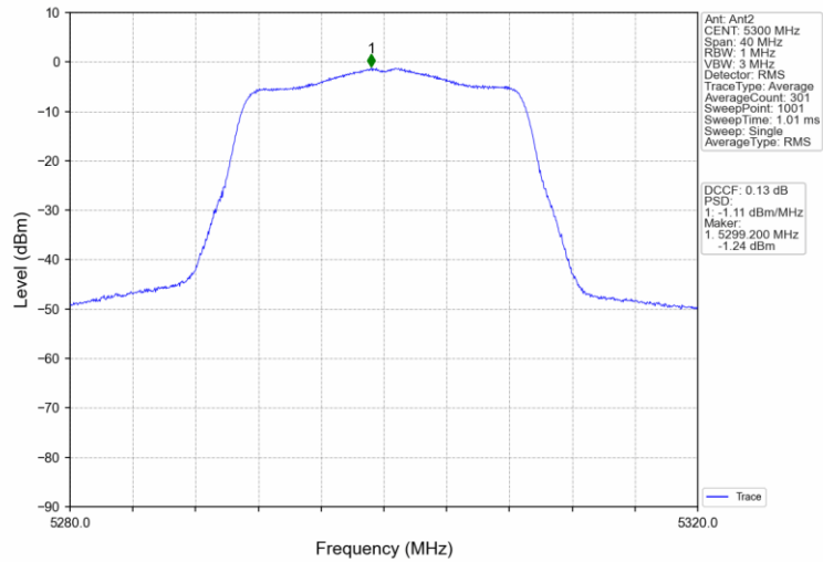
802.11ac(VHT20)_MCH_5300MHz_MIMO_NTNV
