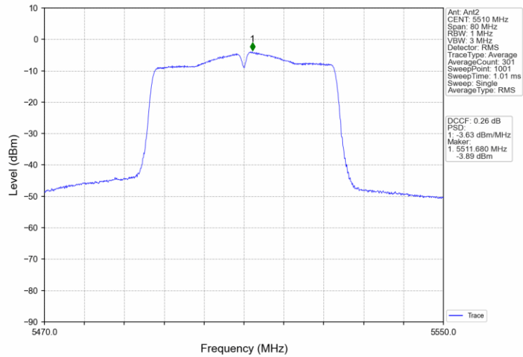
802.11ac(VHT40)_LCH_5510MHz_MIMO_NTNV
