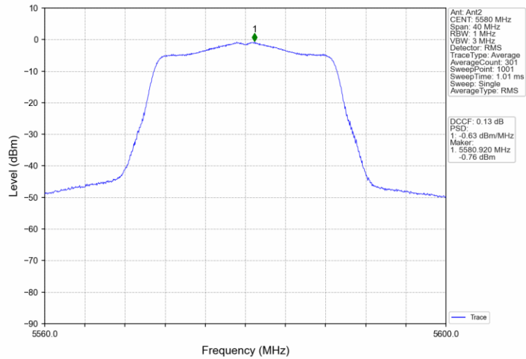
802.11ac(VHT20)_MCH_5580MHz_MIMO_NTNV
