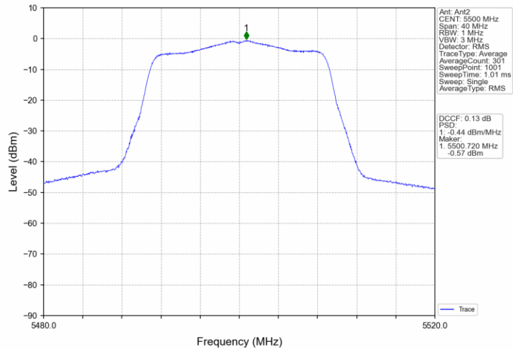
802.11ac(VHT20)_LCH_5500MHz_MIMO_NTNV
