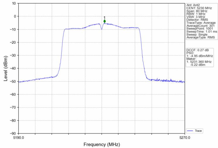
802.11ac(VHT40)_HCH_5230MHz_MIMO_NTNV
