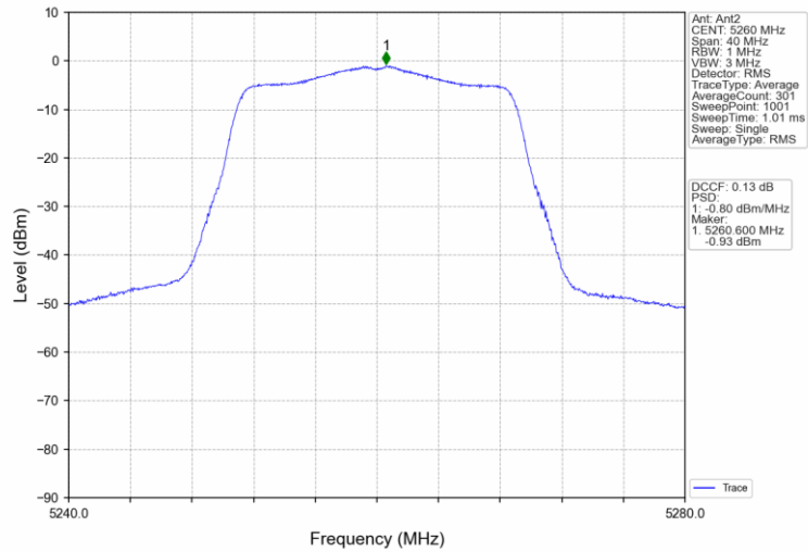
802.11ac(VHT20)_LCH_5260MHz_MIMO_NTNV
