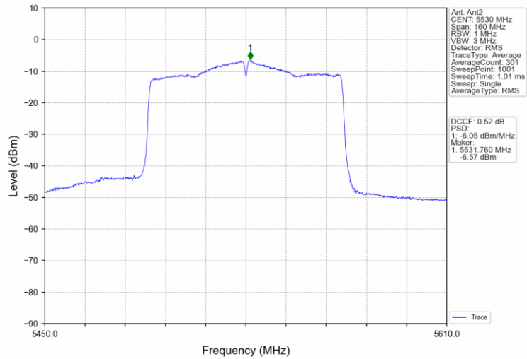
802.11ac(VHT80)_LCH_5530MHz_MIMO_NTNV
