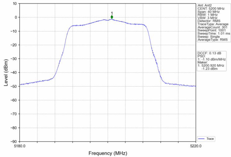
802.11ac(VHT20)_MCH_5200MHz_MIMO_NTNV
