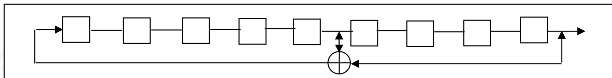
Linier Feedback Shift Register for Generator of the PRBS sequence
