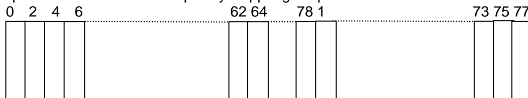
Linier Feedback Shift Register for Generator of the PRBS sequence
