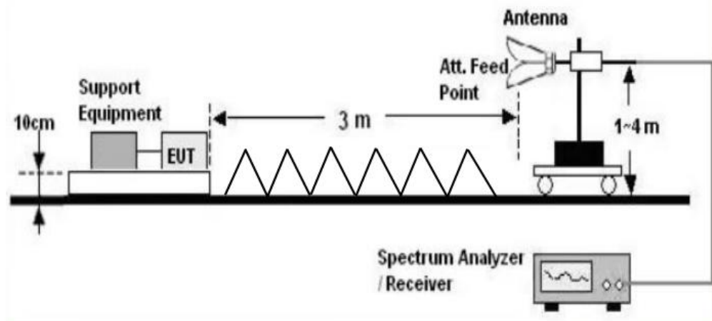
Figure 3. Above 1 GHz
