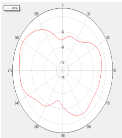
Phi=90 Freq=2420MHz
