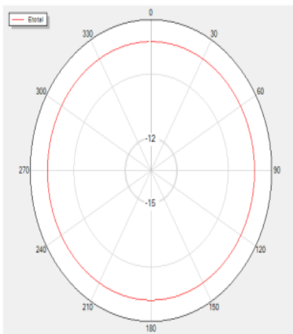
Theta=0 Freq=2420MHz
