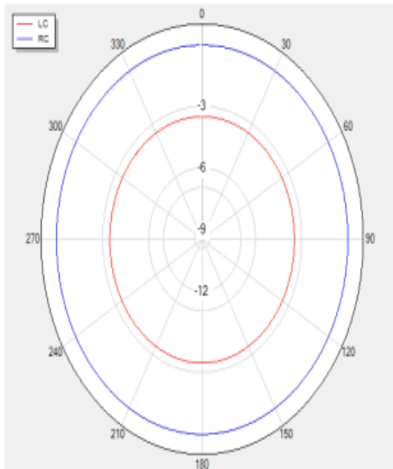
Theta=0 freq=2420MHz
