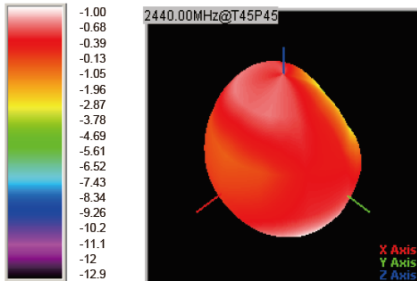
© 3D Gain Pattern (2440 MHz) Unit:dBi
