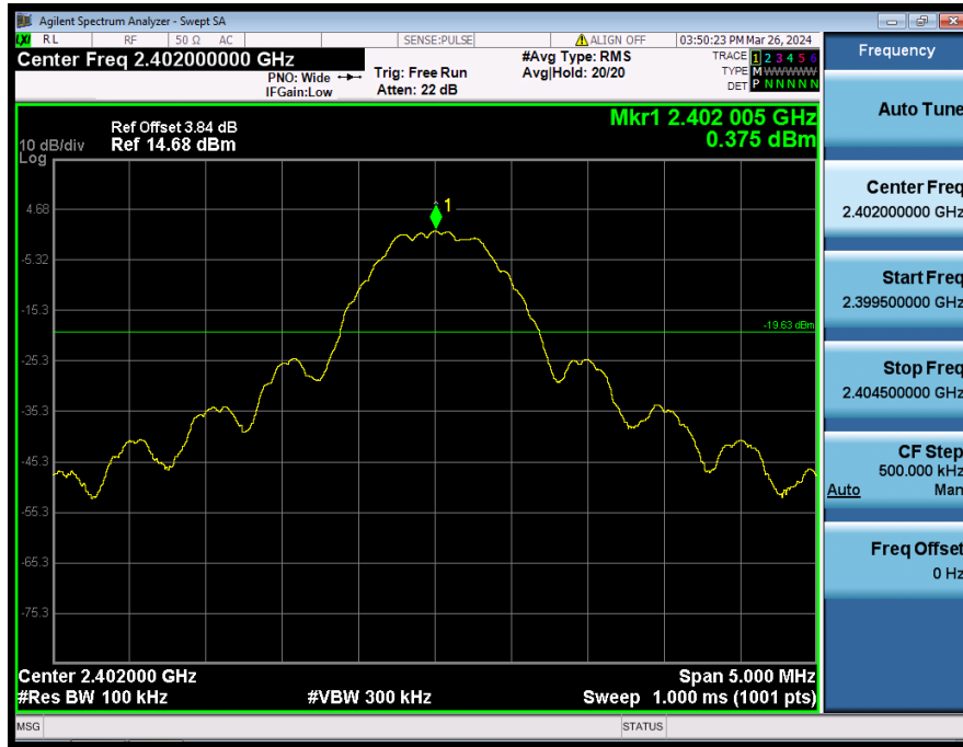
2_Bandedge_NVNT_ANT1_GFSK_2402
