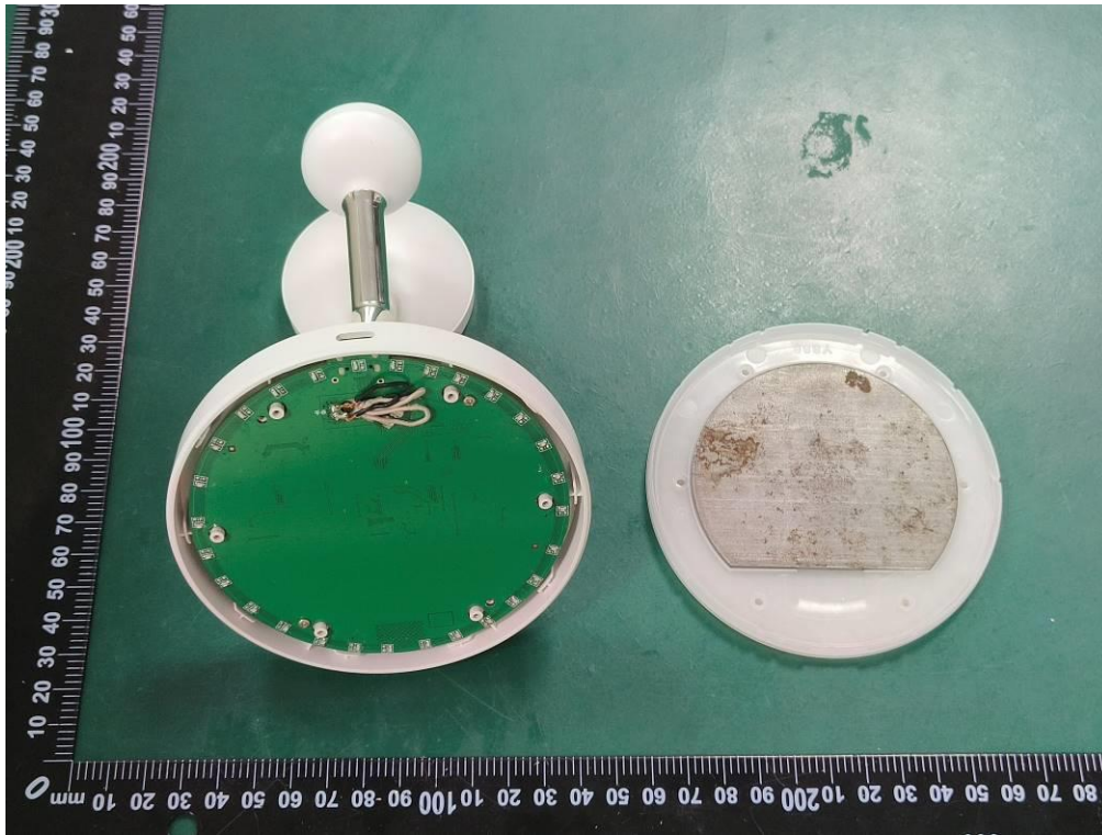
Internal Photo FCC ID: 2BDND-Y888
