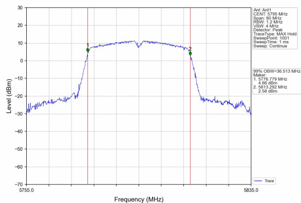
(802.11 n40) channel 159
