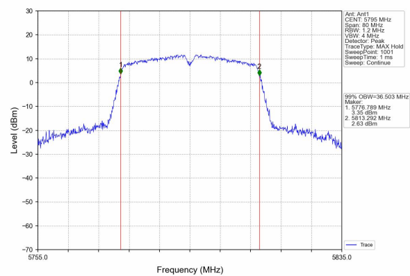
(802.11 ac40) channel 159
