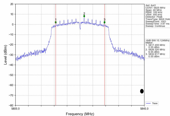
(802.11ac20) 6dB Bandwidth plot on channel 165
