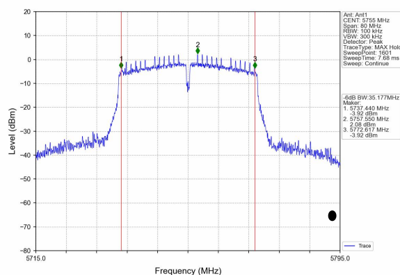
(802.11 n40) 6dB Bandwidth plot on channel 151
