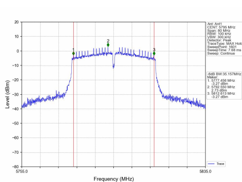
(802.11 ac40) 6dB Bandwidth plot on channel 159
