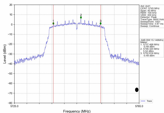
(802.11n20) 6dB Bandwidth plot on channel 149
