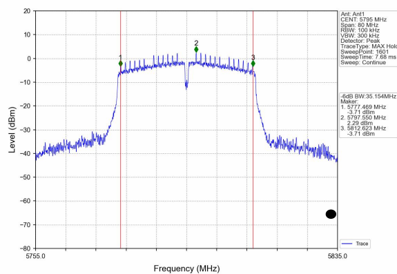
(802.11 n40) 6dB Bandwidth plot on channel 159
