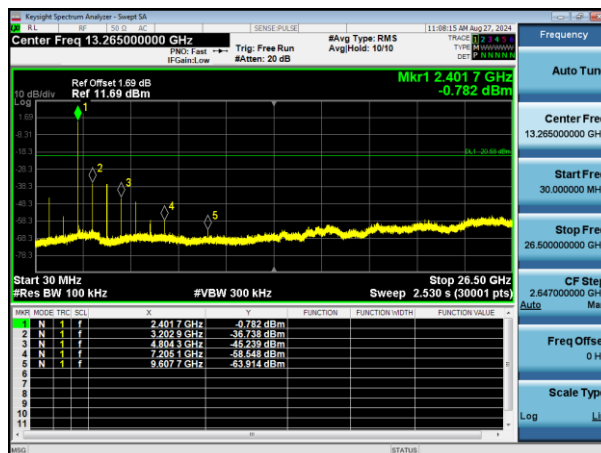
Spurious Emissions
