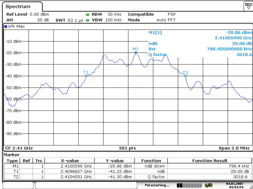
Ant1-2410
