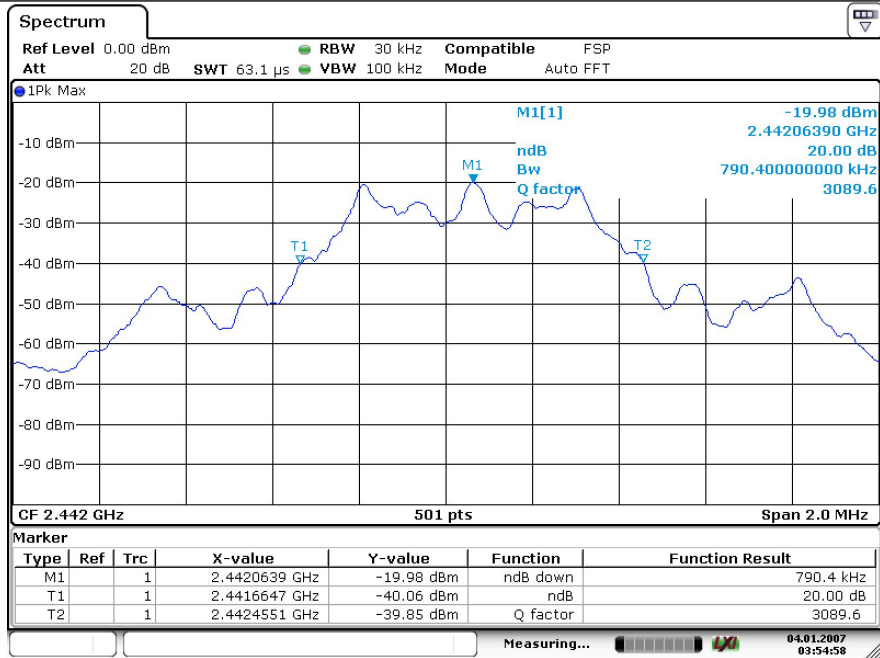
Ant1-2442
