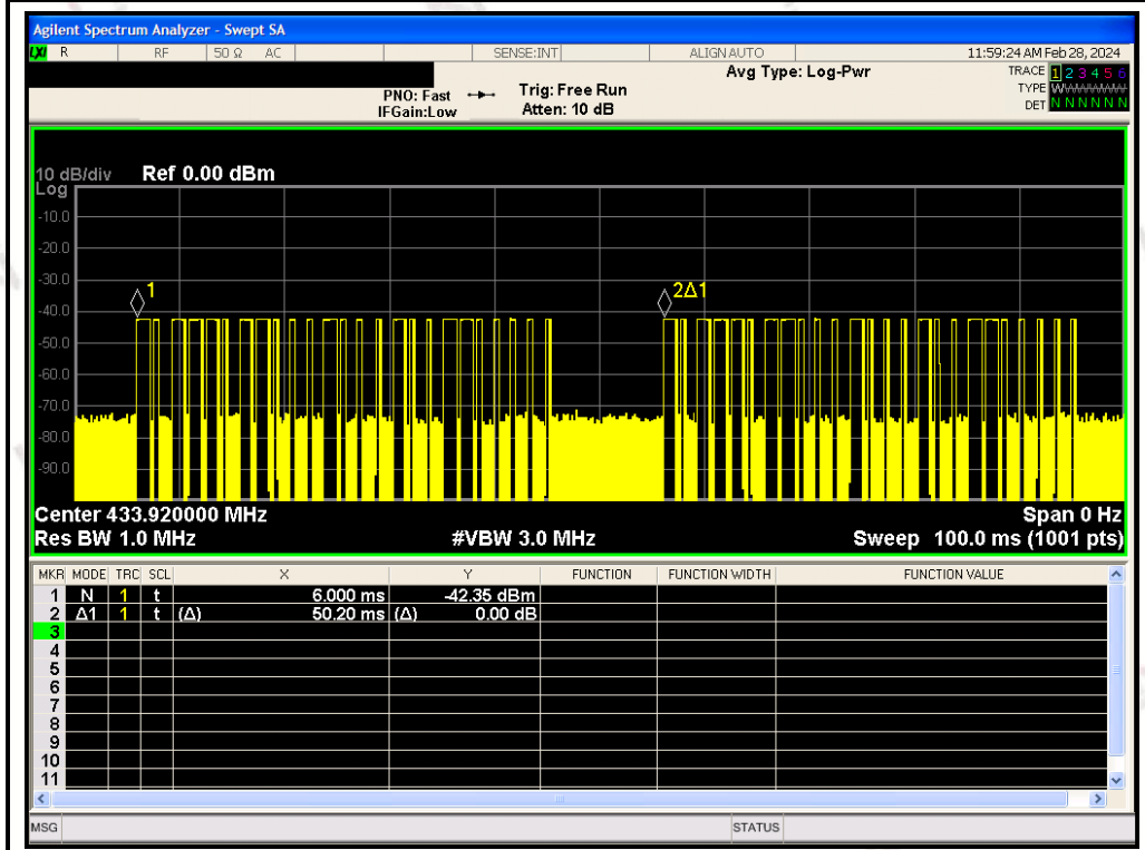
T_{on} + T_{off}
