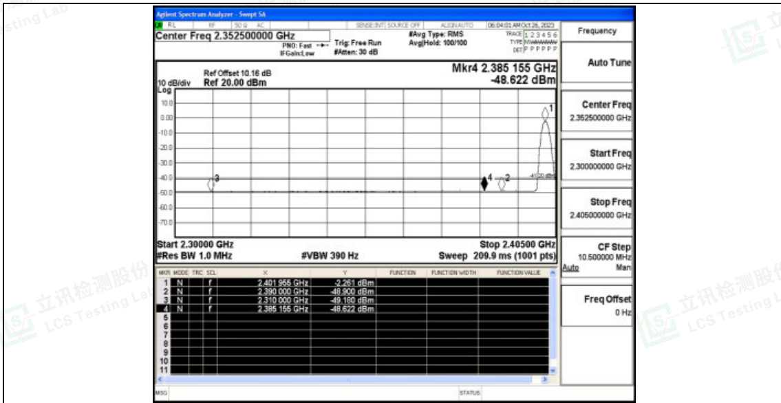
2DH5_Ant1_Low_2402_Peak
