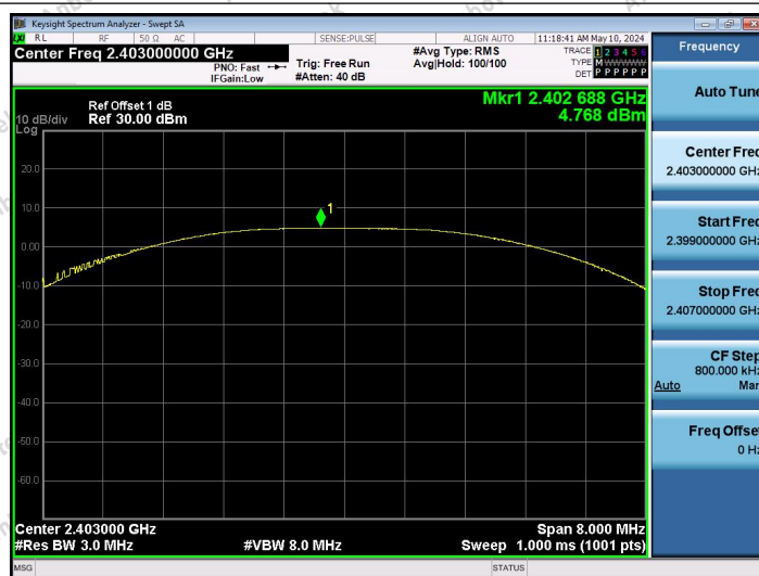
2.4G-Ant1-2403-PASS
