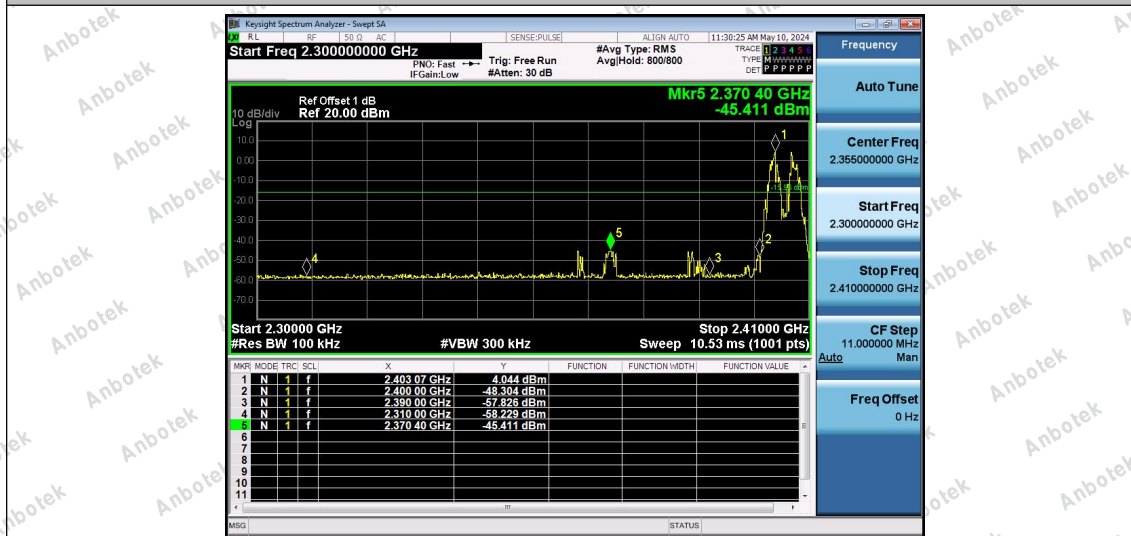
2.4G-Ant1-Hop_2403-PASS
