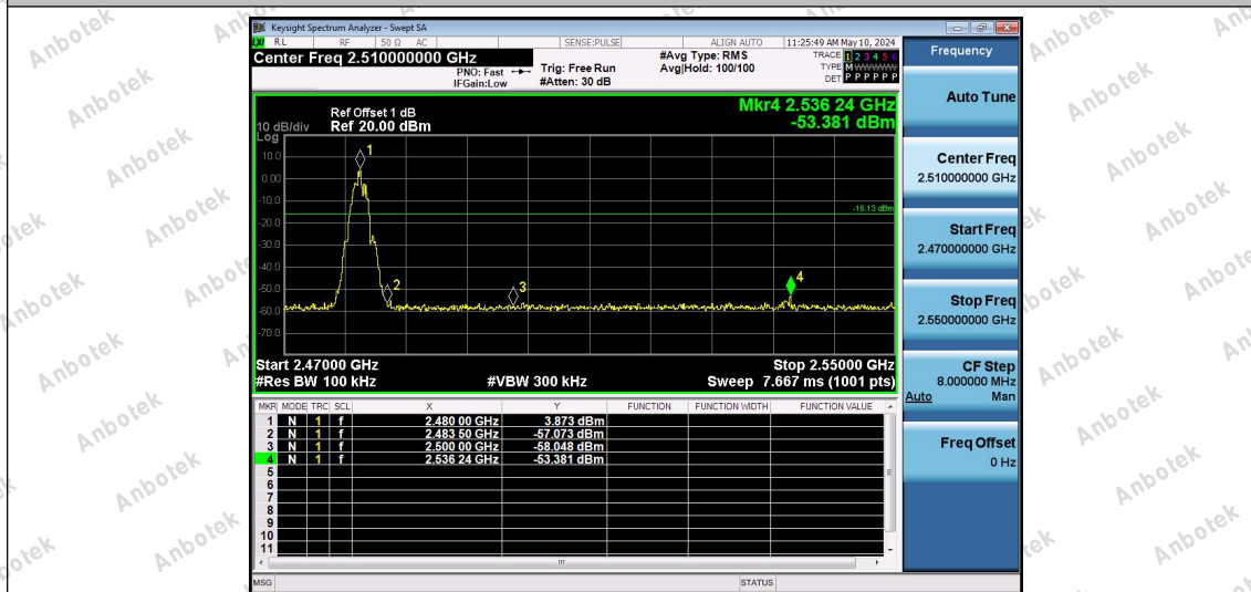
2.4G-Ant1-2480-PASS
