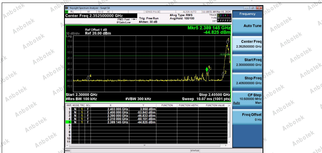
2.4G-Ant1-2403-PASS
