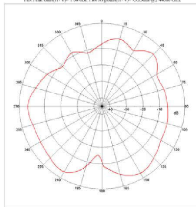
Far-field Power Distribution(H+V) on X-Z Plane Plot Peak Gain(H+V)= 1.08 dB; Plot AvgGain(H+V)= -3.83dB @2.44000 GHz
