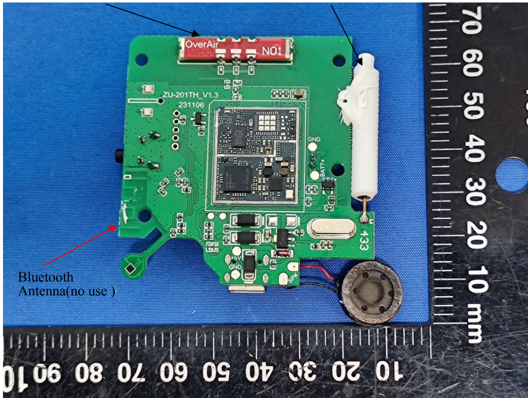
NB-IoT Antenna 433.92MHz Rx Antenna
