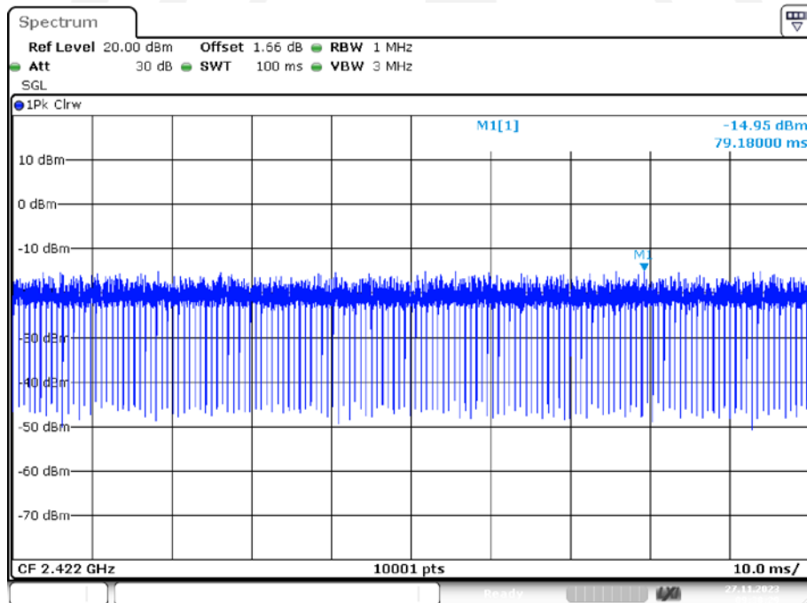
IEEE 802.11 n/HT40 2422MHz
