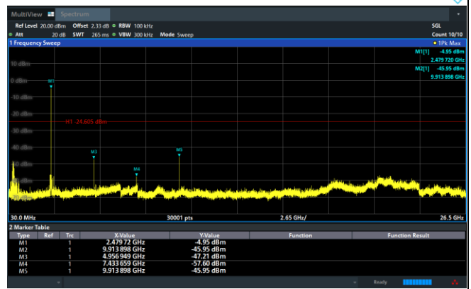
GFSK on Channel 78
