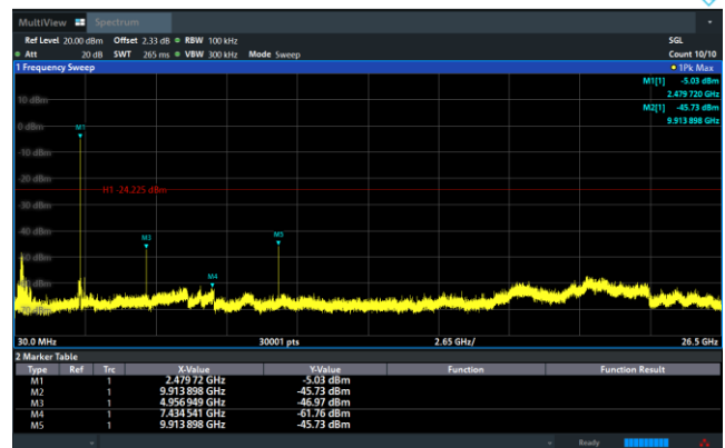
\pi/4 -DQPSK on Channel 78
