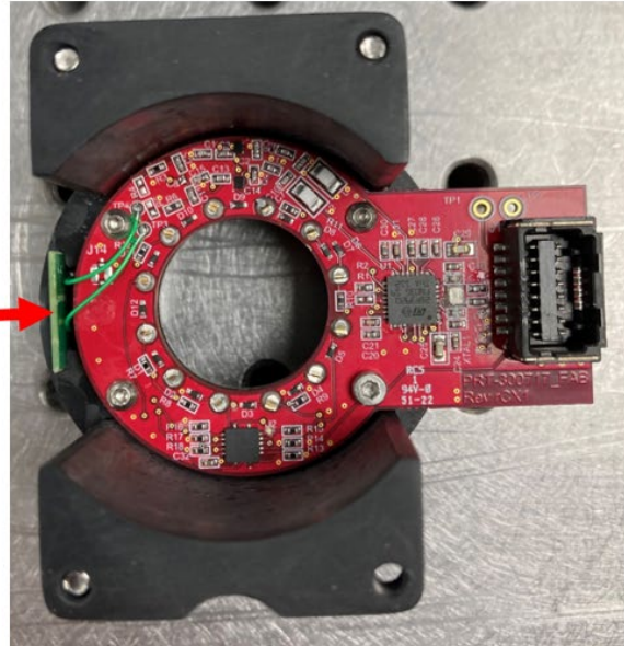
NFC Antenna attached to NFC board
