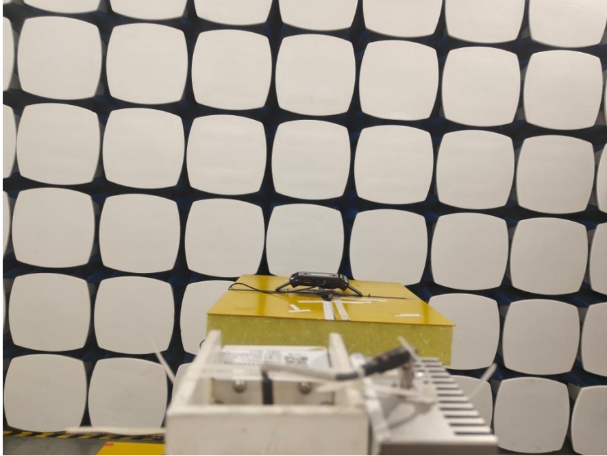
Radiated Spurious Emission: 18GHz-40GHz
