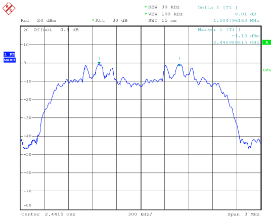
8DPSK_Middle 1.005 MHz
