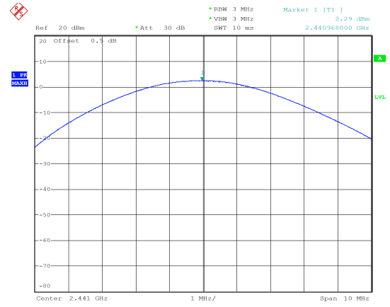
PI/4-DQPSK_Middle 2.29 dBm
