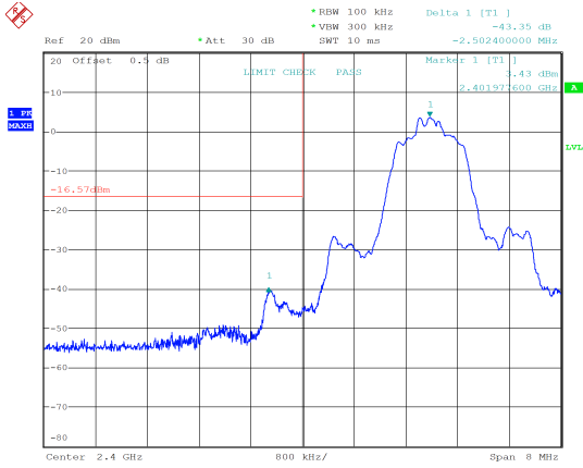
PI/4-DQPSK_Low 43.35 dB
