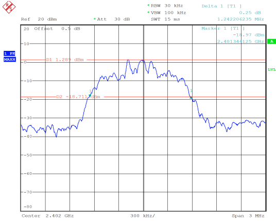
PI/4-DQPSK_Low 1.242 MHz
