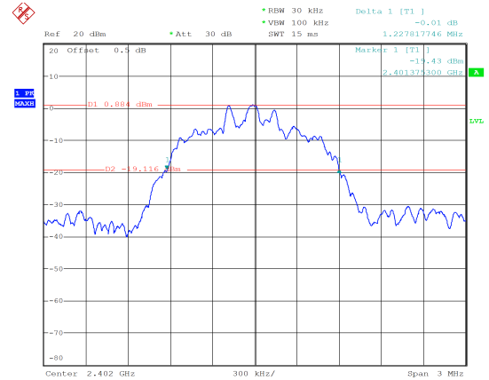
8DPSK_Low 1.228 MHz
