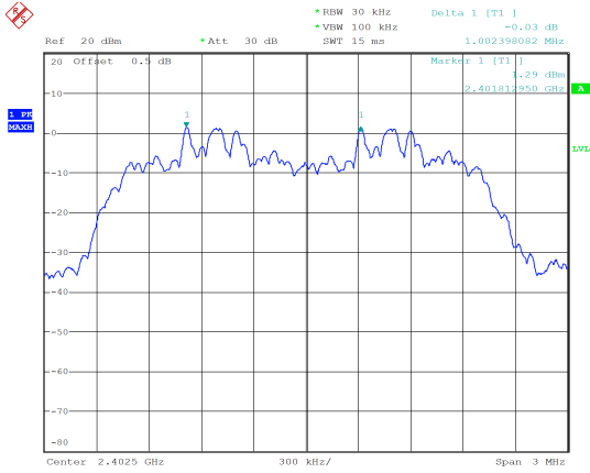
PI/4-DQPSK_Low 1.002 MHz
