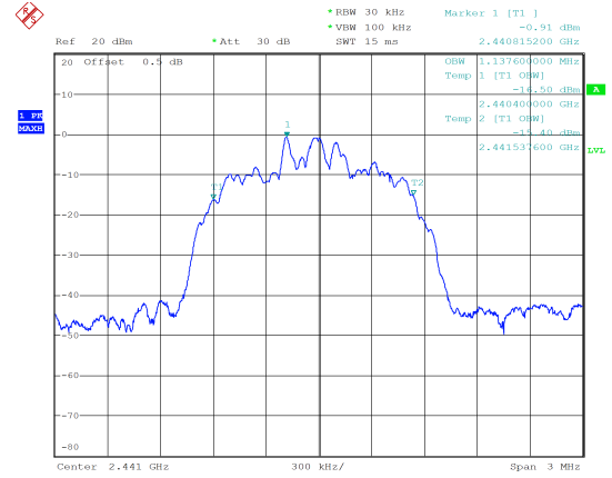
PI/4-DQPSK_Middle 1.138 MHz
