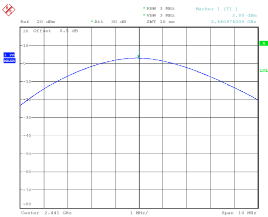
8DPSK_Middle 2.80 dBm
