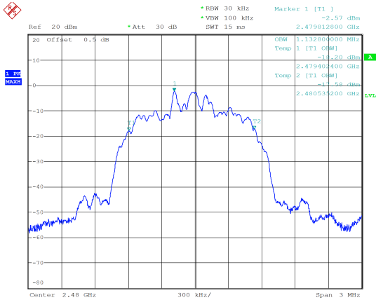
PI/4-DQPSK_High 1.133 MHz
