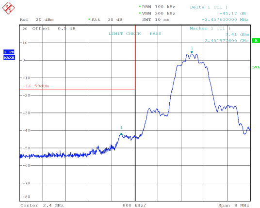
8DPSK_Low 45.17 dB
