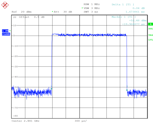
8DPSK_Hopping_3DH3 1.674ms
