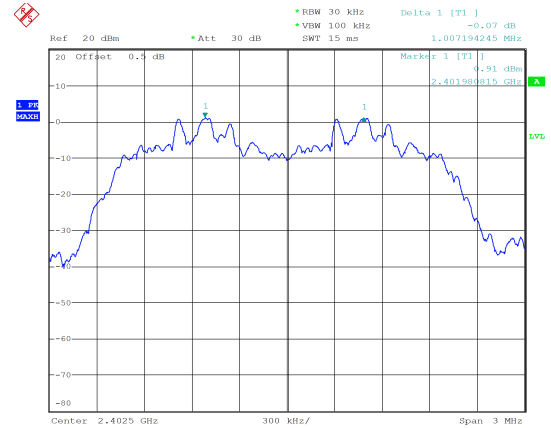
8DPSK_Low 1.007 MHz
