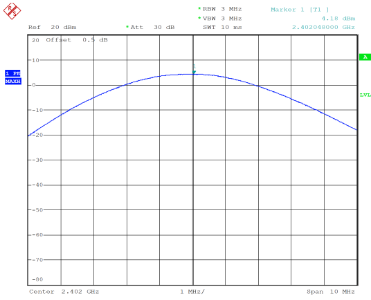
PI/4-DQPSK_Low 4.18 dBm
