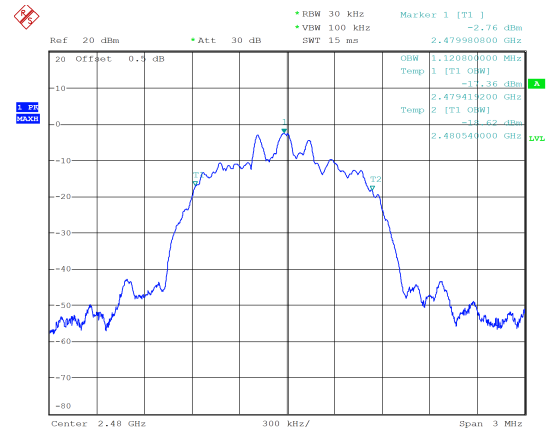
8DPSK_High 1.121 MHz
