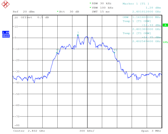
PI/4-DQPSK_Low 1.162 MHz
