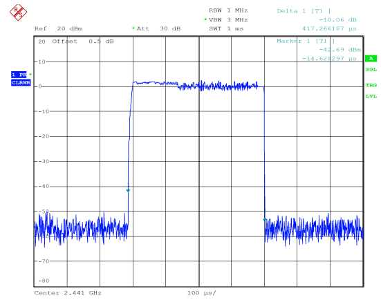
8DPSK_Hopping_3DH1 0.417ms
