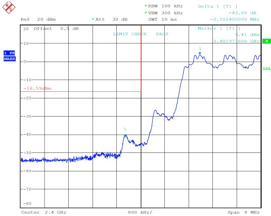
PI/4-DQPSK_Hopping_Lower 43.80 dB
