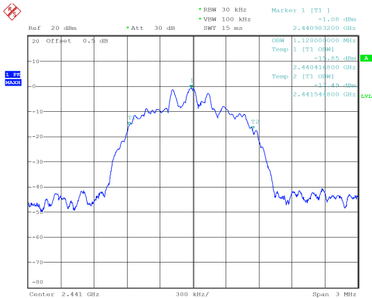
8DPSK_Middle 1.128 MHz
