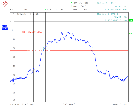
PI/4-DQPSK_High 1.240 MHz
