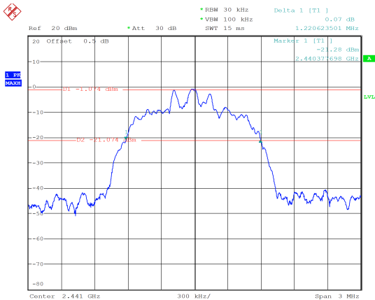
8DPSK_Middle 1.221 MHz
