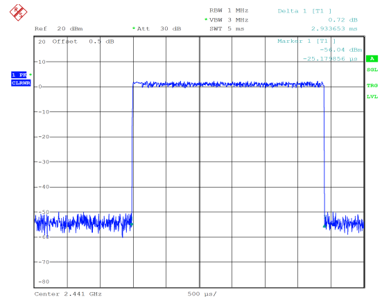
8DPSK_Hopping_3DH5 2.934ms
