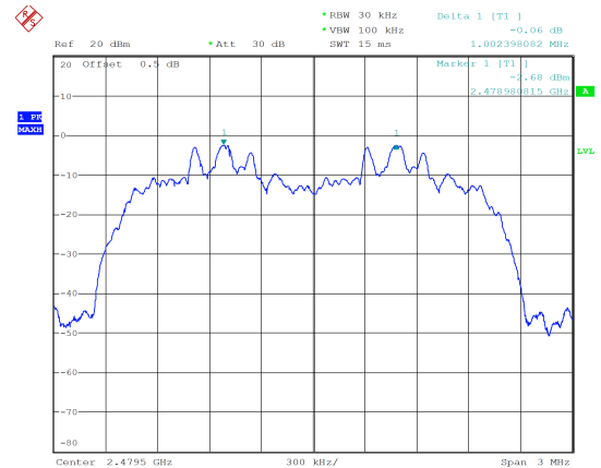
8DPSK_High 1.002 MHz
