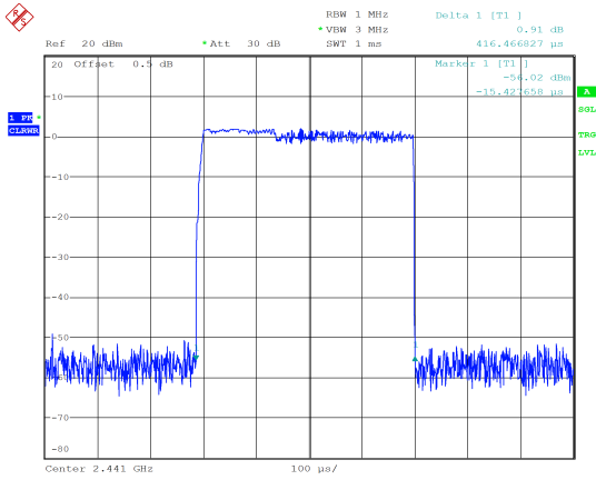
PI/4-DQPSK_Hopping_2DH1 0.416ms
