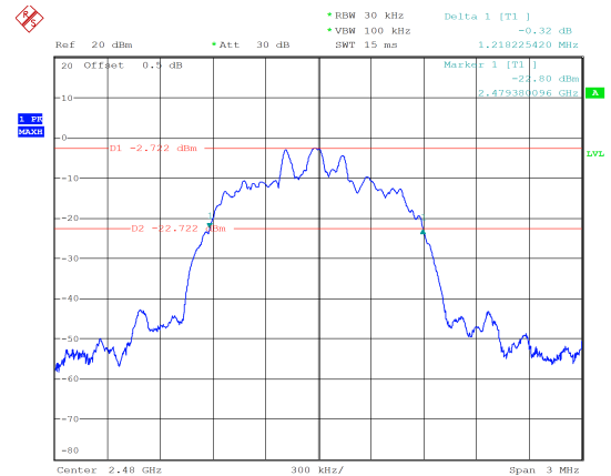
8DPSK_High 1.218 MHz
