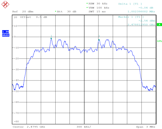
PI/4-DQPSK_High 1.002 MHz
