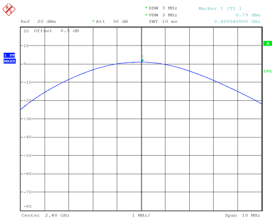
PI/4-DQPSK_High 0.79 dBm
