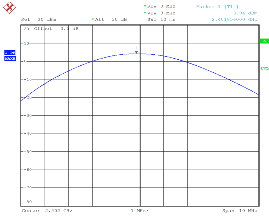
GFSK_Low 3.94 dBm
