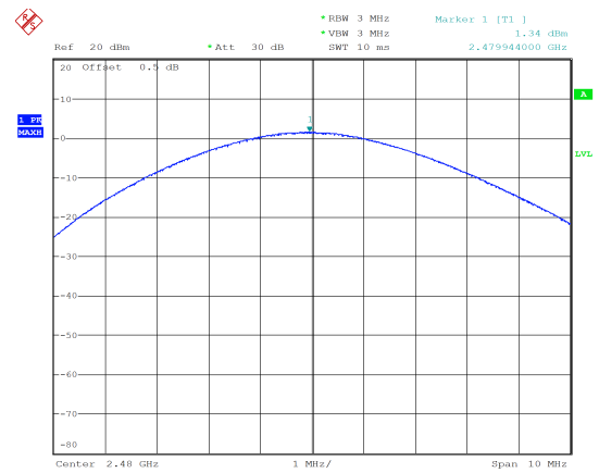
8DPSK_High 1.34 dBm
