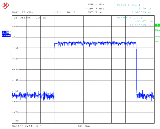
PI/4-DQPSK_Hopping_2DH5 2.926ms
