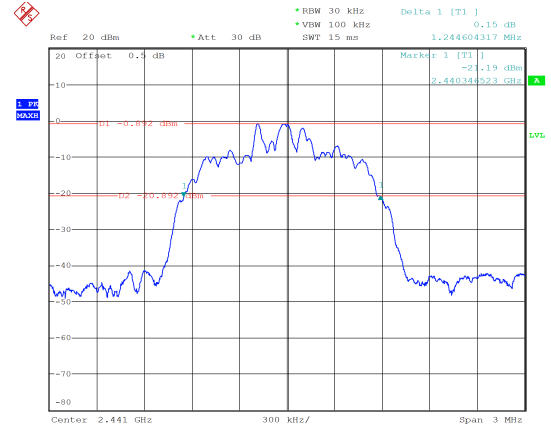
PI/4-DQPSK_Middle 1.245 MHz
