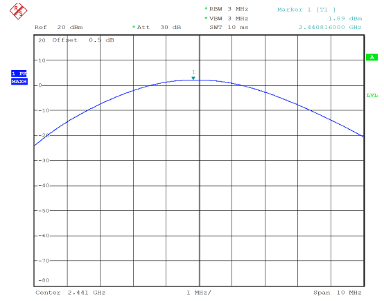
GFSK_Middle 1.89 dBm
