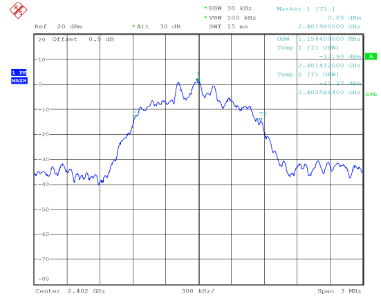
8DPSK_Low 1.154 MHz
