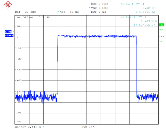
PI/4-DQPSK_Hopping_2DH3 1.674ms
