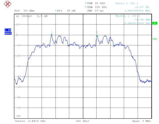
PI/4-DQPSK_Middle 1.002 MHz
