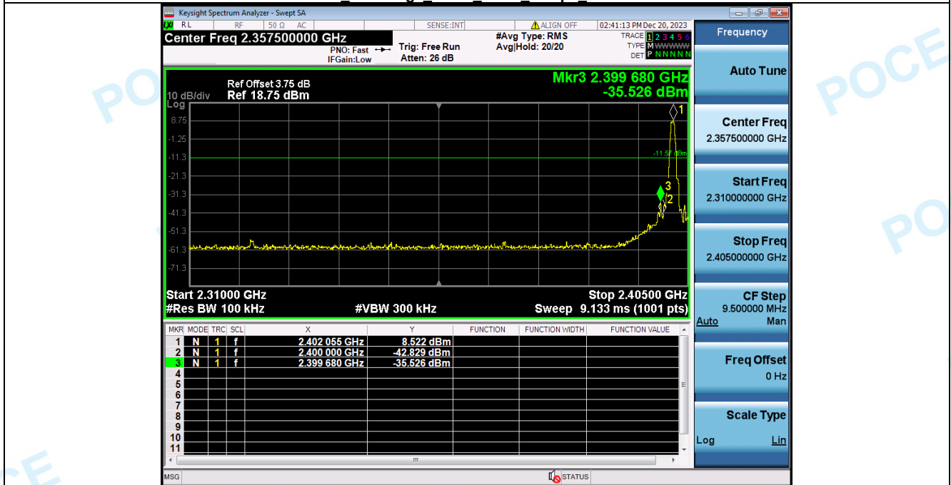
2 Bandedge NVNT_ANT1_1Mbps_2402
