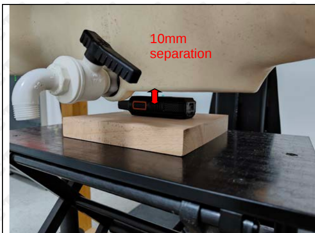
Hotspot(Front side)
